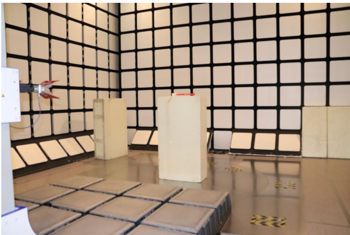
Photograph 4. Radiated emissions 1 – 10 GHz
