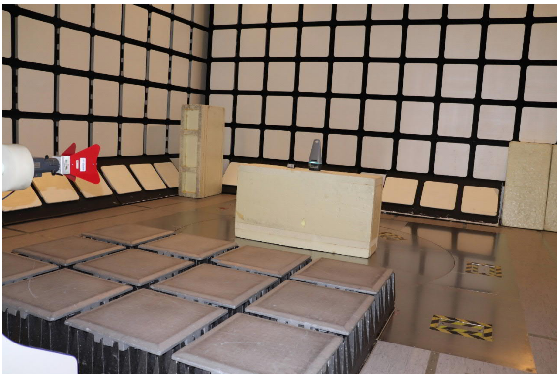
Photograph 6. Radiated emissions 1 – 10 GHz
