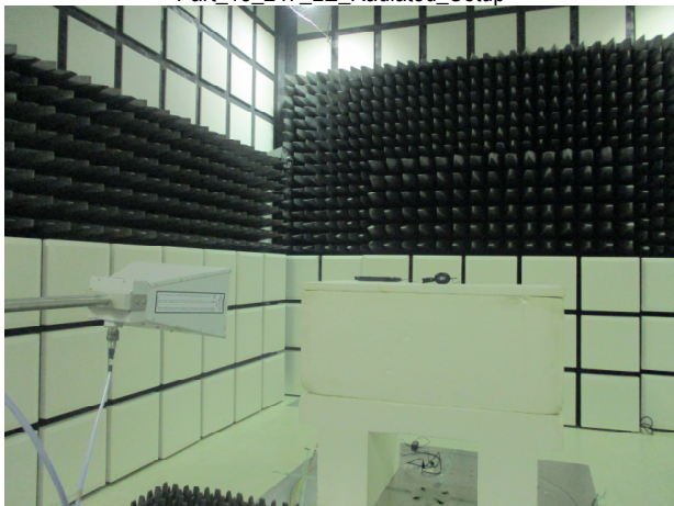
Part_15_247_LE_Radiated_Setup
