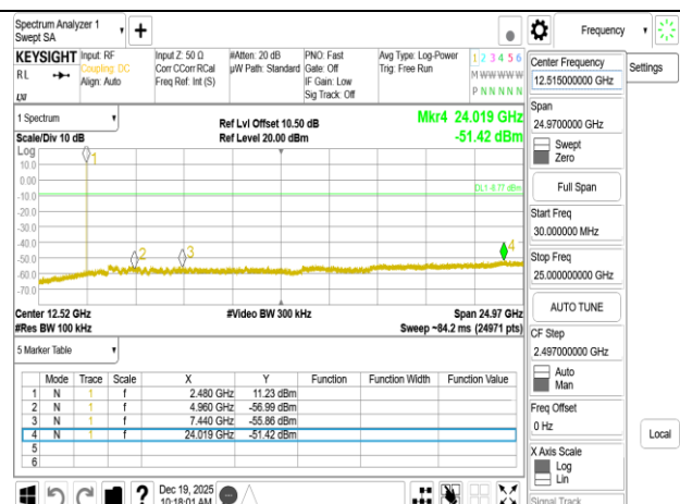
Spurious Emission \pi/4 DQPSK 2M DH5 2480MHz
