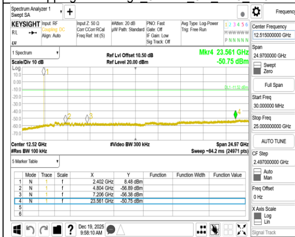
Spurious Emission GFSK 1M DH5 2402MHz
