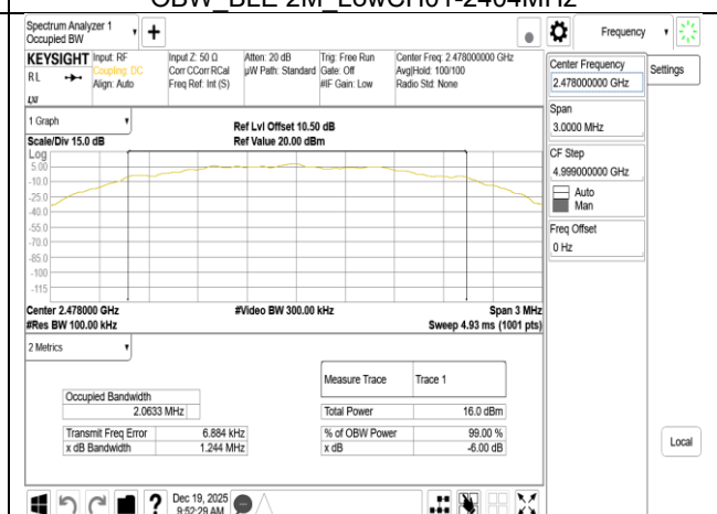
OBW_BLE 2M_HighCH38-2478MHz
