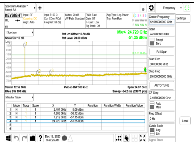
Spurious Emission_BLE 2M_LowCH01-2404MHz
