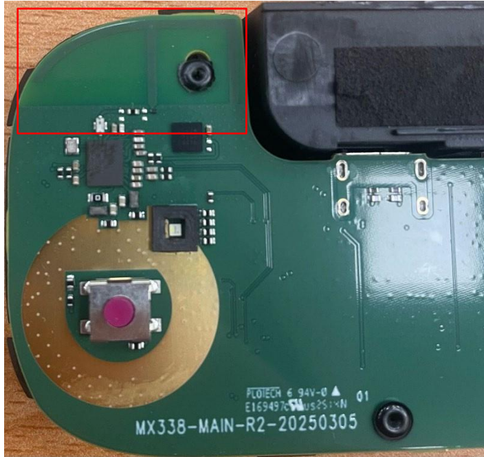
MX338 Antenna Pattern
