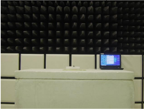
FCC_15_247_BT_Radiated_Setup
