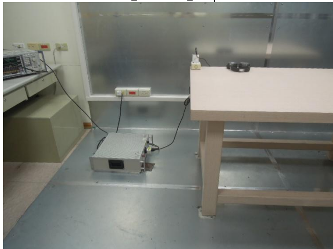
BT_Conduction_Setup
