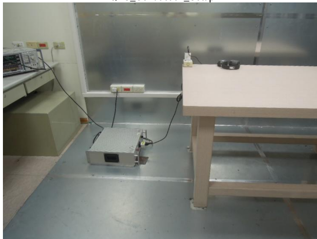
QHS_Conduction_Setup
