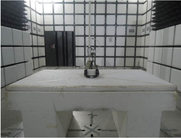
BT_Radiated_1 st _Setup
