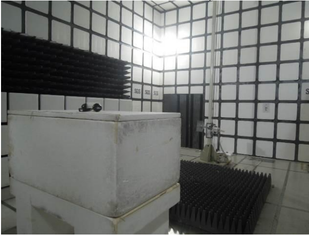
QHS_Radiated_1st_Setup
