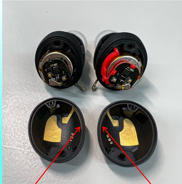
Left Earbud Antenna
