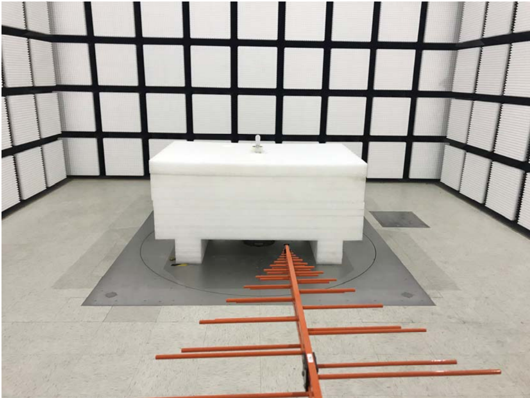
Radiated Emissions Below 1G View
