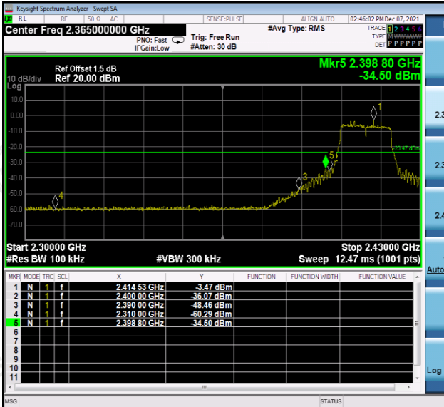
Left bandedge
