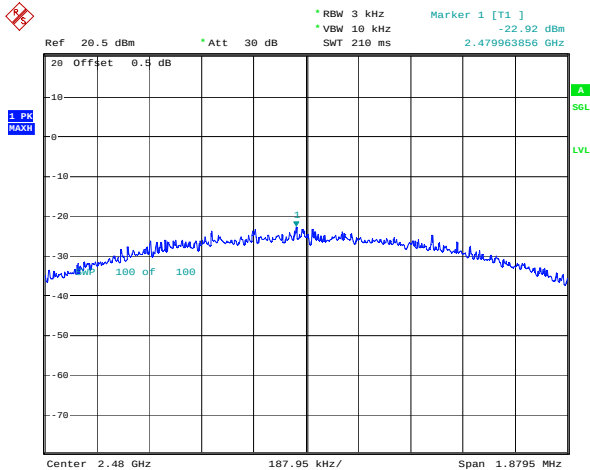
BLE_2M_High_Channel
