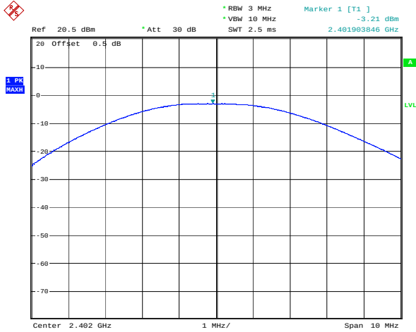
BLE_2M_Low_Channel
