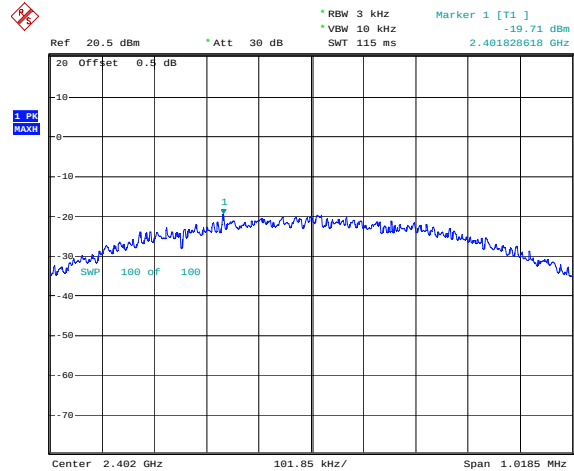
BLE_1M_Low_Channel
