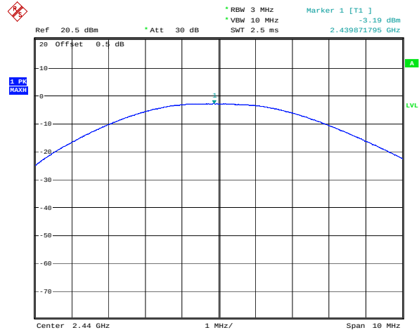
BLE_2M_Middle_Channel
