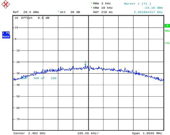
BLE_2M_Low_Channel
