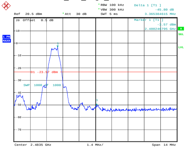
BLE_1M_High_Channel
