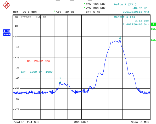
BLE_1M_Low_Channel
