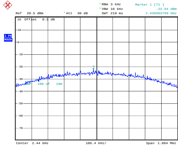
BLE_2M_Middle_Channel
