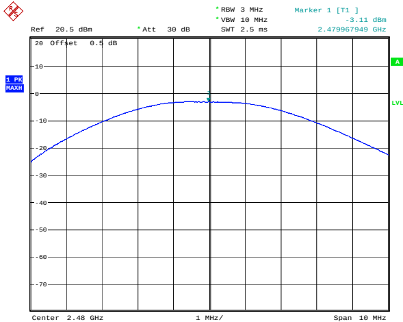
BLE_2M_High_Channel
