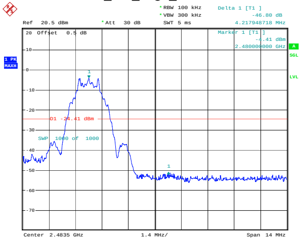
BLE_2M_High_Channel
