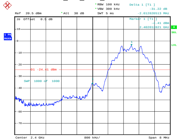
BLE_2M_Low_Channel
