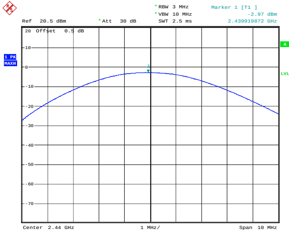
BLE_1M_Middle_Channel
