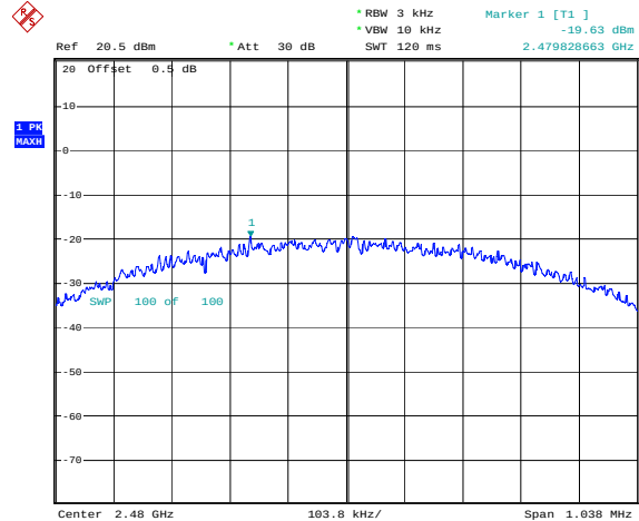
BLE_1M_High_Channel
