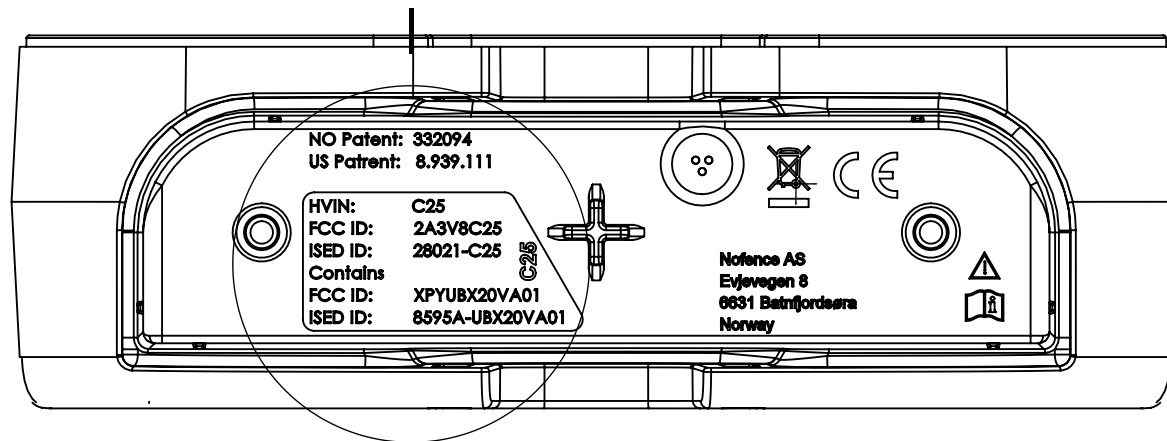
DETAIL 1 SCALE 2 : 1
