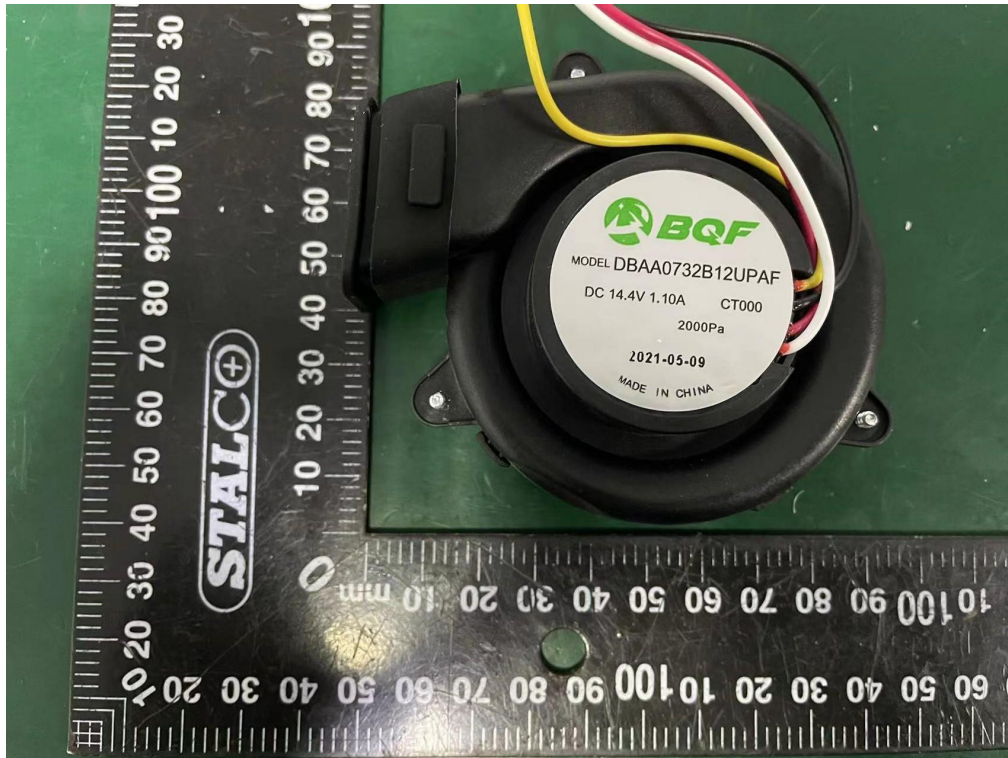
Internal Photos M/N: GRV-3011
