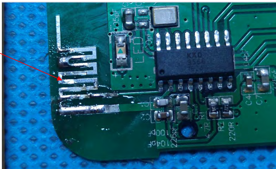
PCB Antenna
