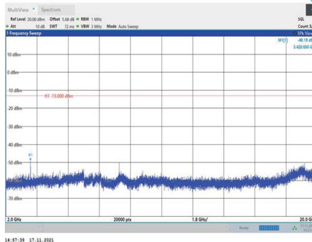
Band4-1.4MHz-QPSK-19957-1RB#0-Range3:2000~20000MHz
