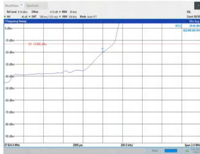
Band5-1.4MHz-QPSK-20643-1RB#0
