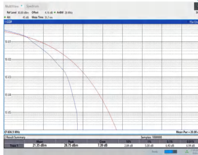
Band5-5MHz-16QAM-20525-25RB#0
