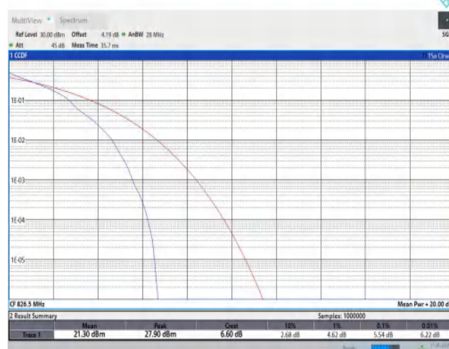
Band5-5MHz-QPSK-20425-1RB#0
