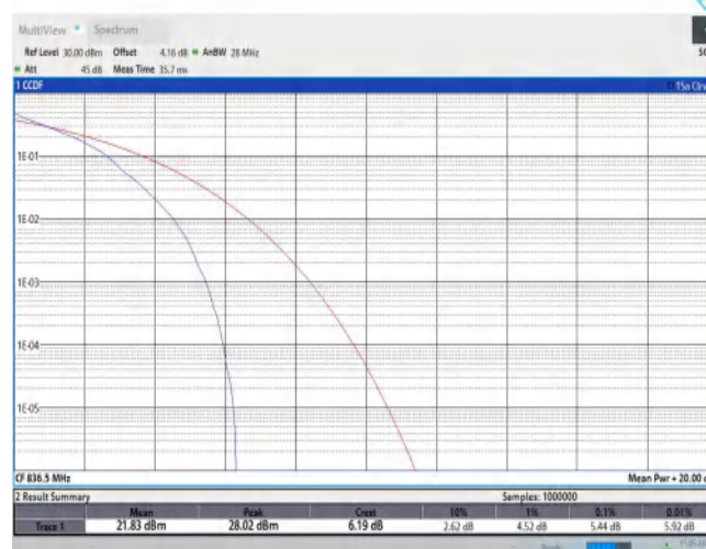
Band5-3MHz-QPSK-20525-1RB#0
