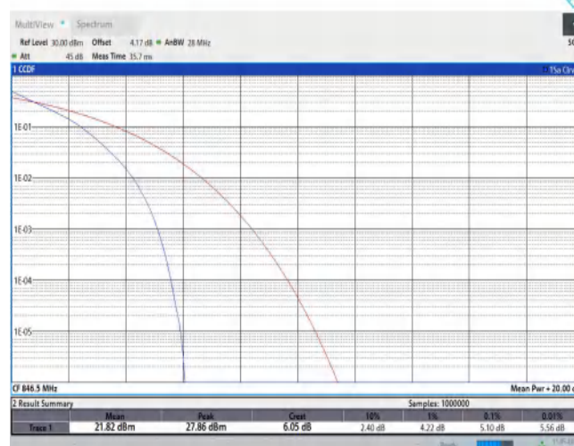
Band5-5MHz-QPSK-20625-25RB#0
