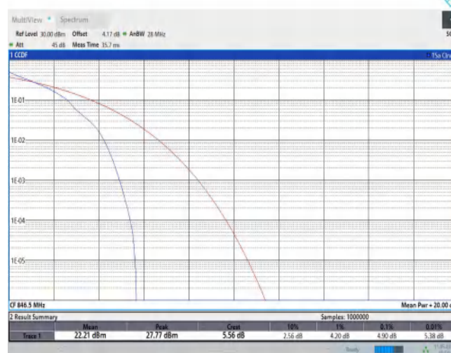
Band5-5MHz-QPSK-20625-25RB#0
