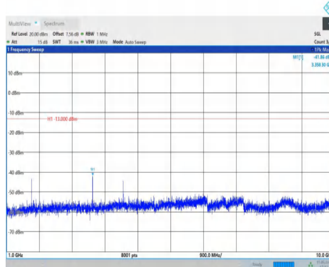
Band5-10MHz-QPSK-20600-1RB#0-Range2:1000~10000MHz
