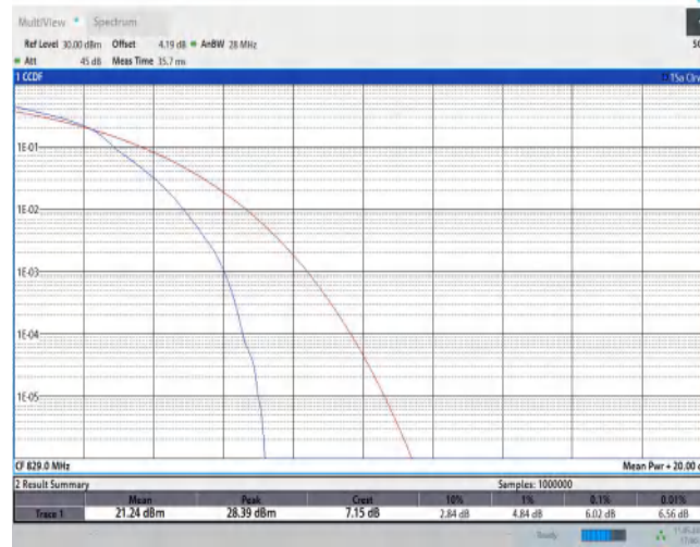
Band5-10MHz-16QAM-20450-50RB#0
