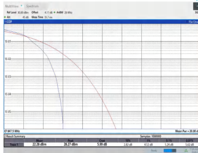
Band5-3MHz-16QAM-20635-15RB#0
