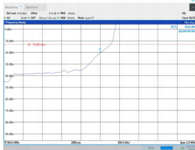
Band5-1.4MHz-QPSK-20407-1RB#5
