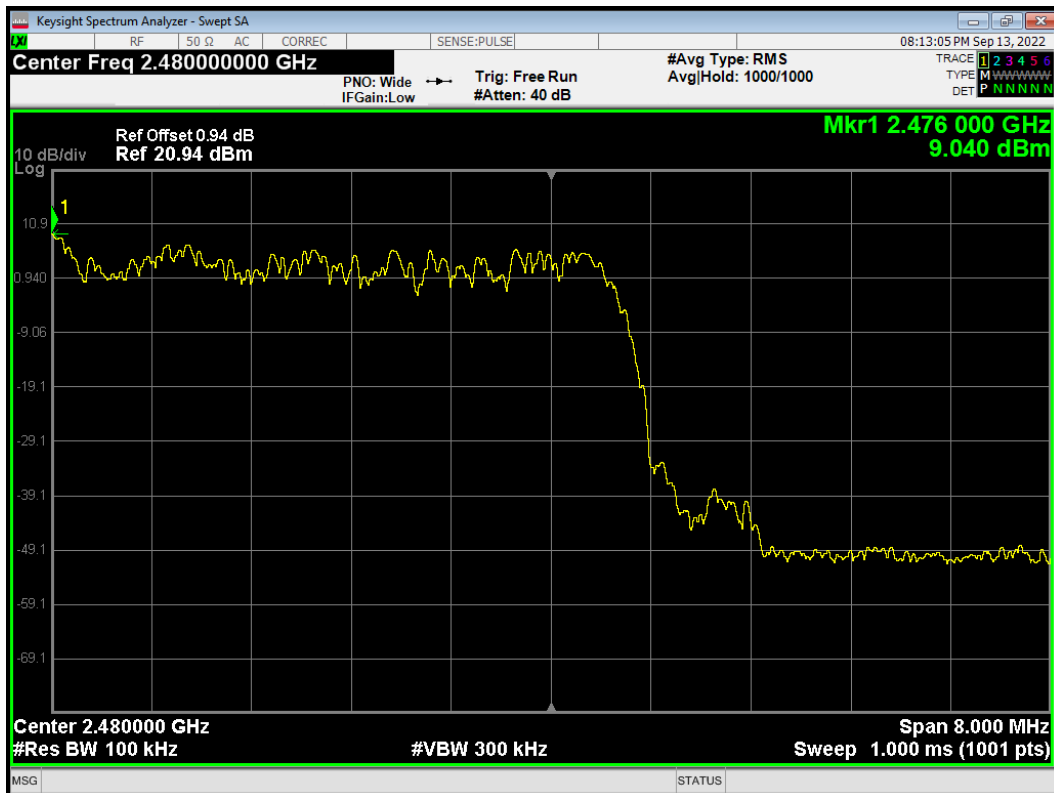
Band Edge(Hopping) 3-DH5 2480MHz Hopping Ref
