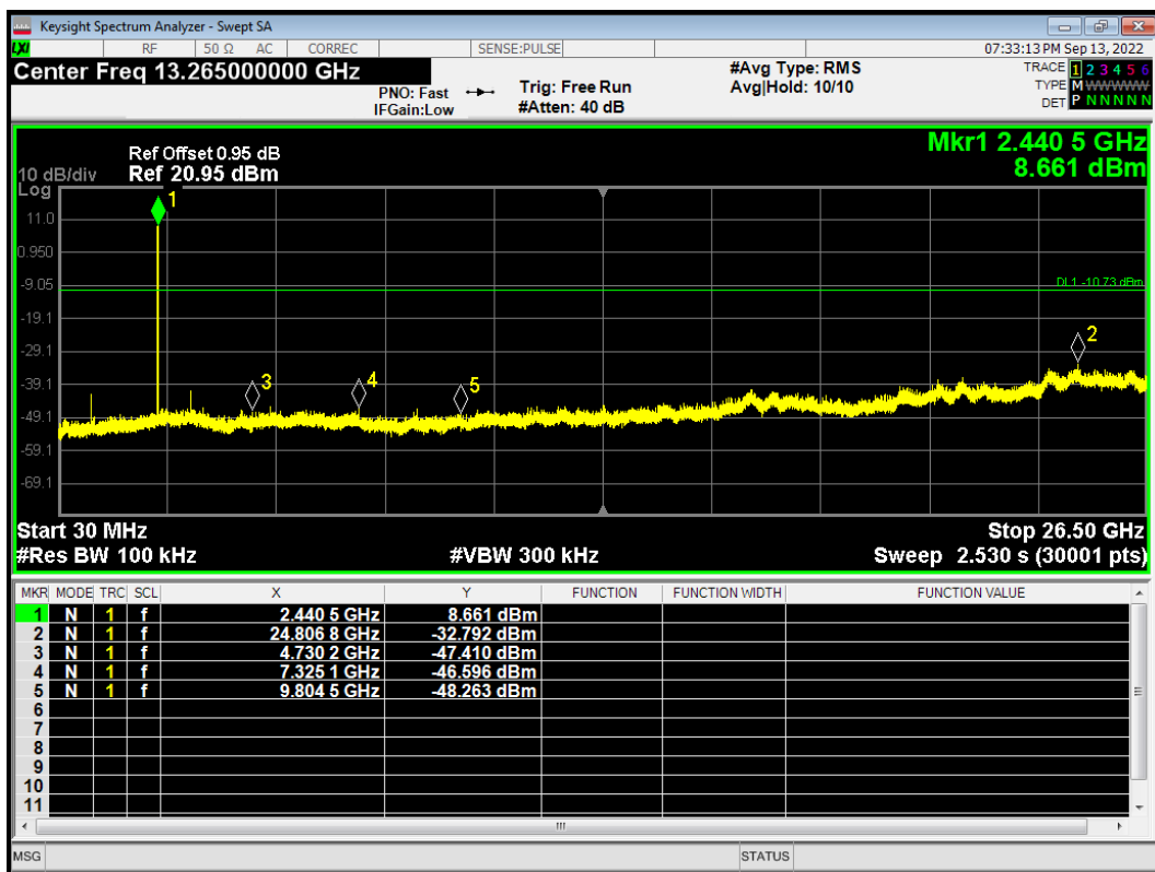
Tx. Spurious 1-DH5 2441MHz Emission
