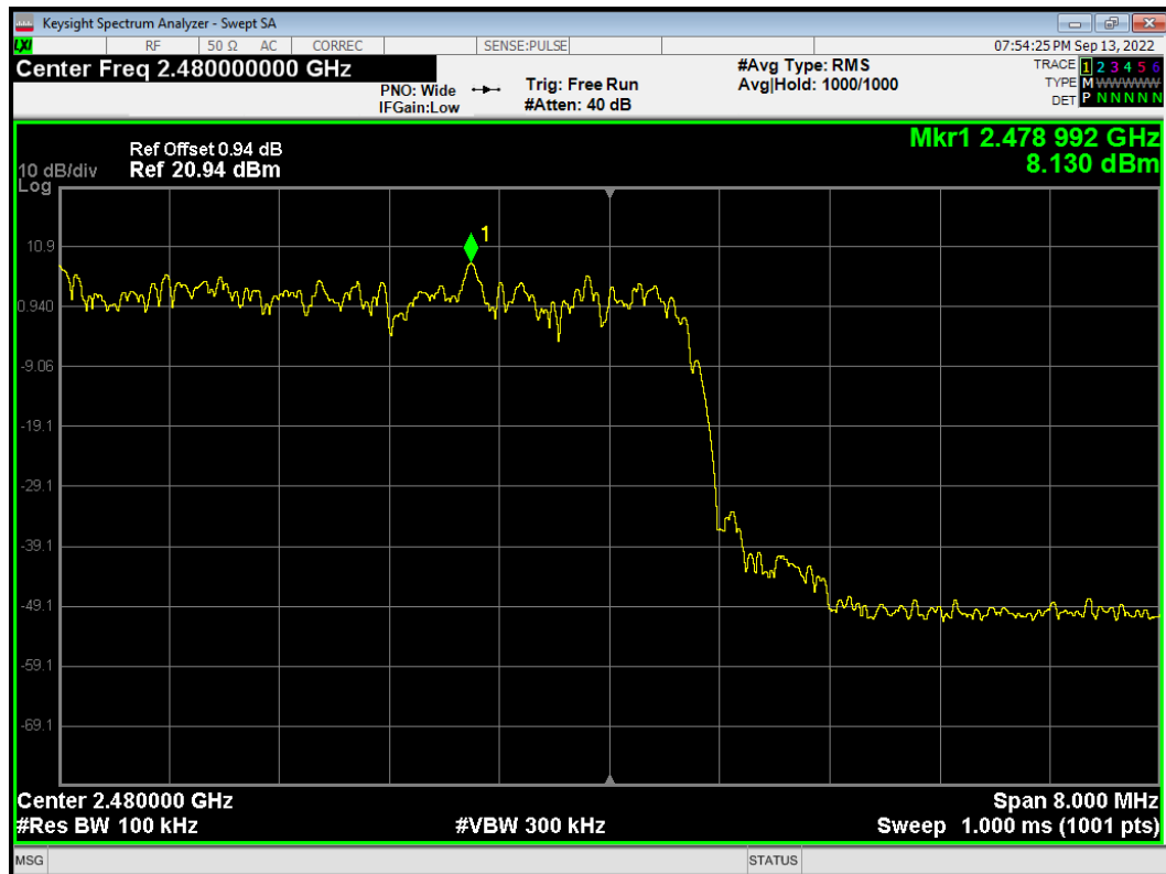
Band Edge(Hopping) 2-DH5 2480MHz Hopping Ref
