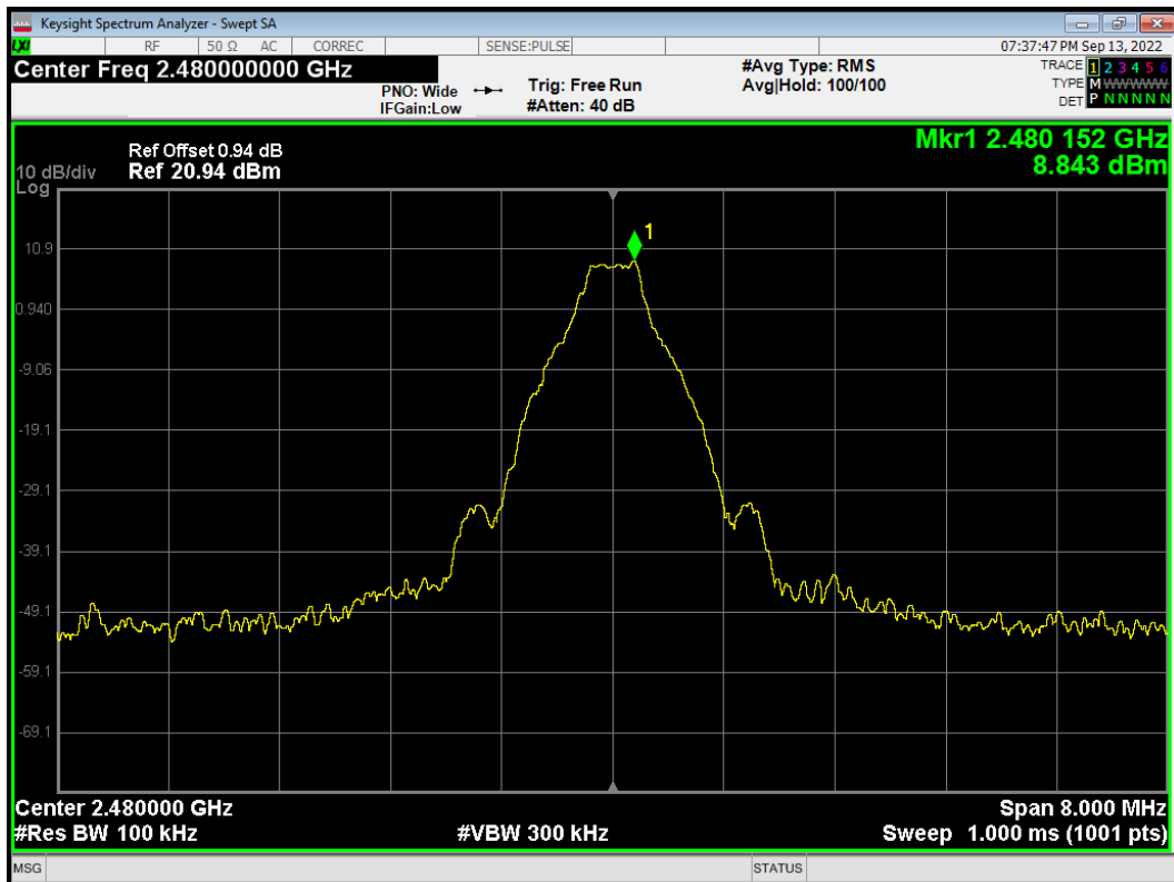
Band Edge 1-DH5 2480MHz No-Hopping Ref
