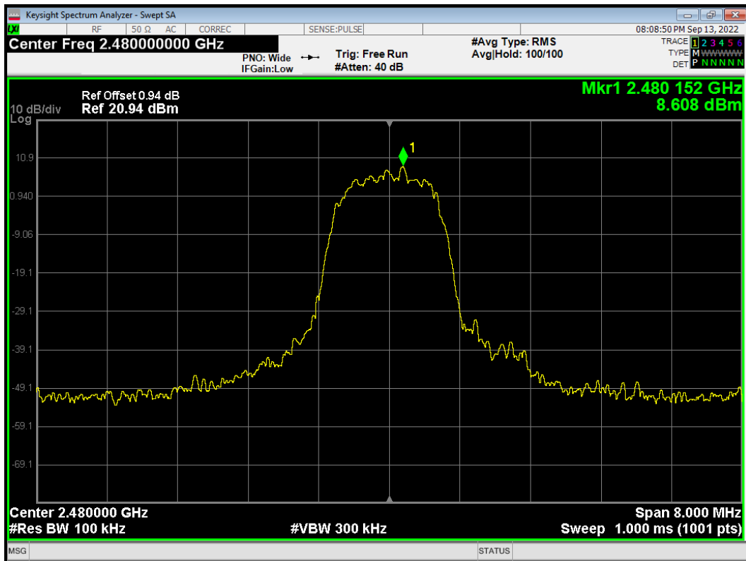
Band Edge 3-DH5 2480MHz No-Hopping Ref
