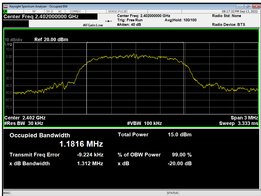
OBW 3-DH5 2402MHz
