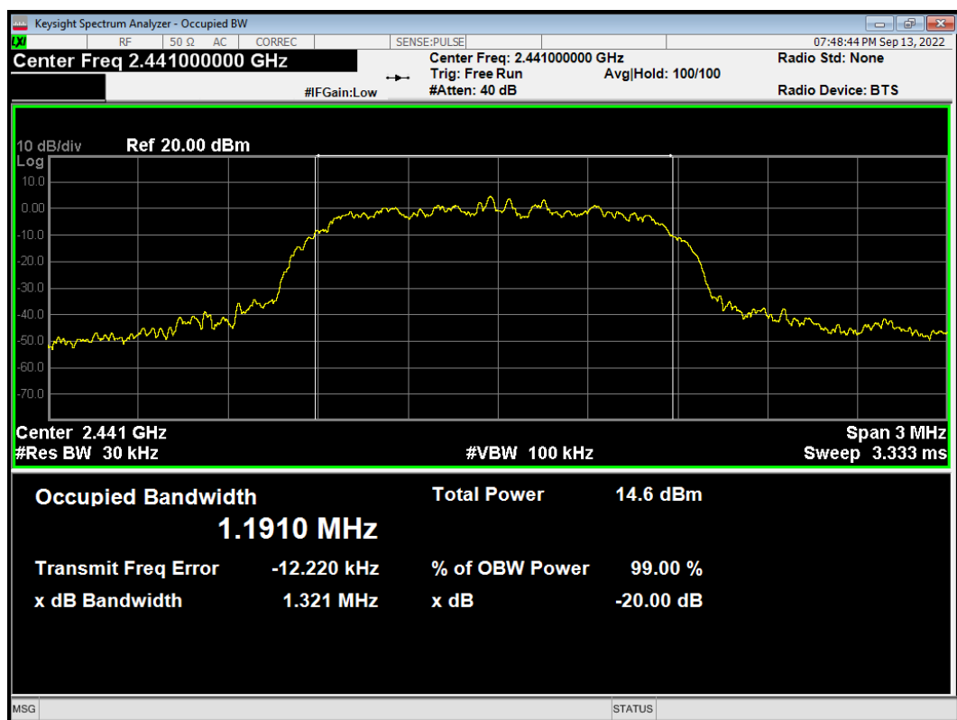
OBW 2-DH5 2441MHz
