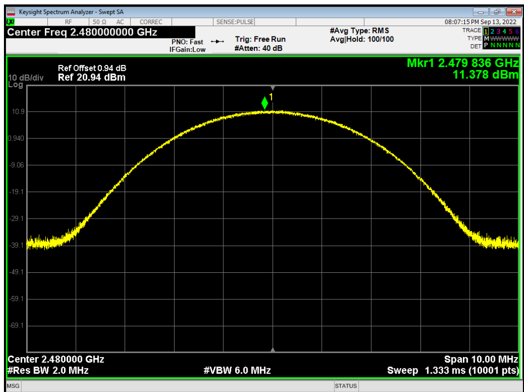
Power 3-DH5 2480MHz
