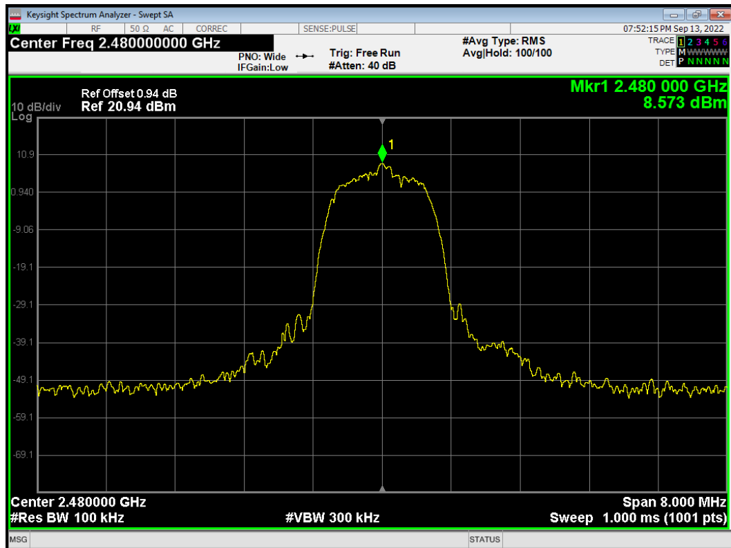
Band Edge 2-DH5 2480MHz No-Hopping Ref
