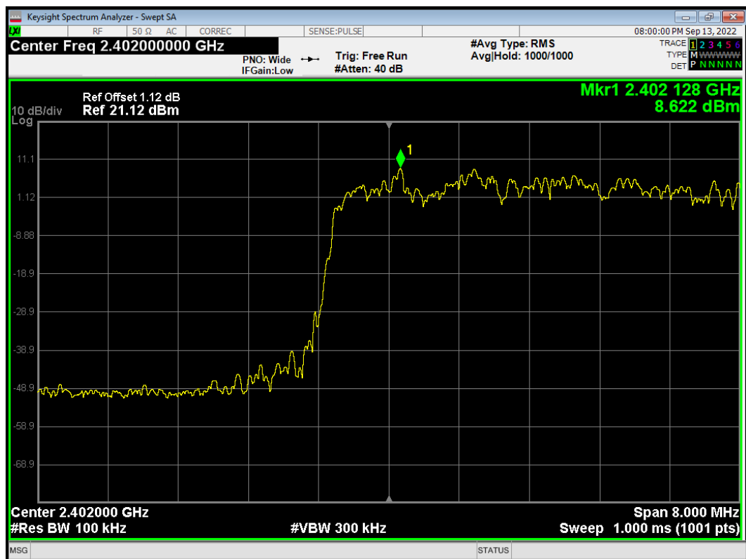
Band Edge(Hopping) 3-DH5 2402MHz Hopping Ref
