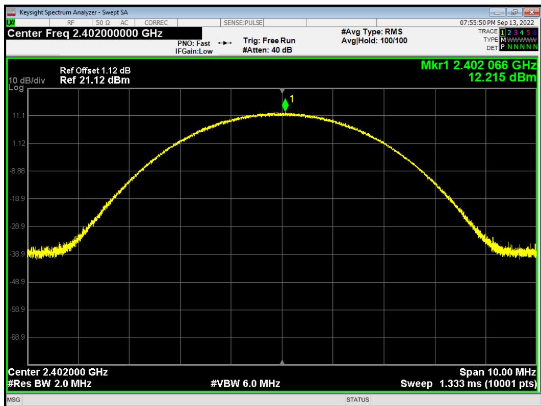
Power 3-DH5 2402MHz
