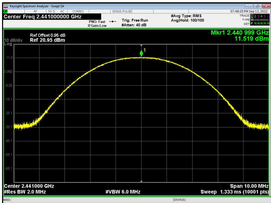
Power 2-DH5 2441MHz
