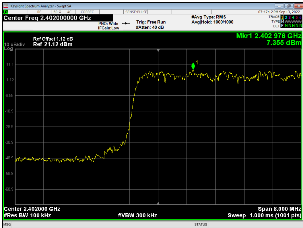
Band Edge(Hopping) 2-DH5 2402MHz Hopping Ref
