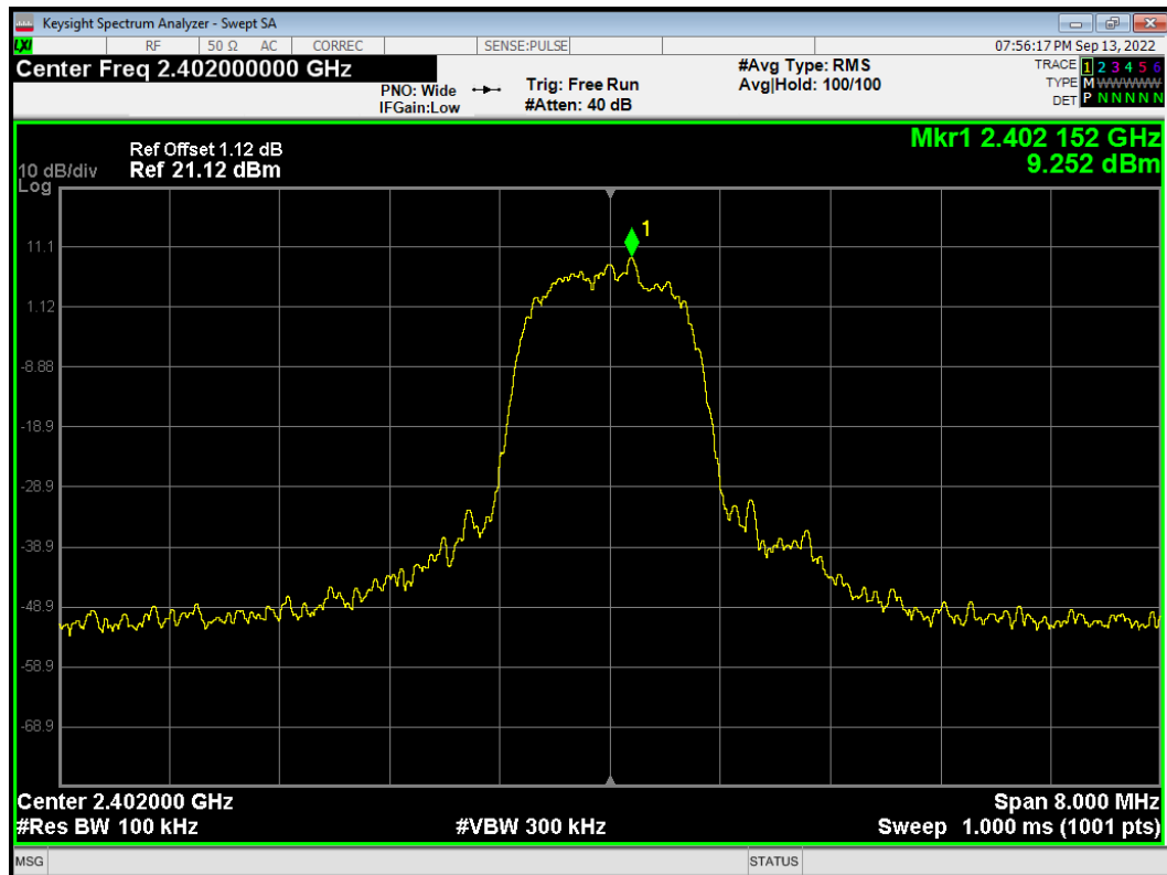
Band Edge 3-DH5 2402MHz No-Hopping Ref
