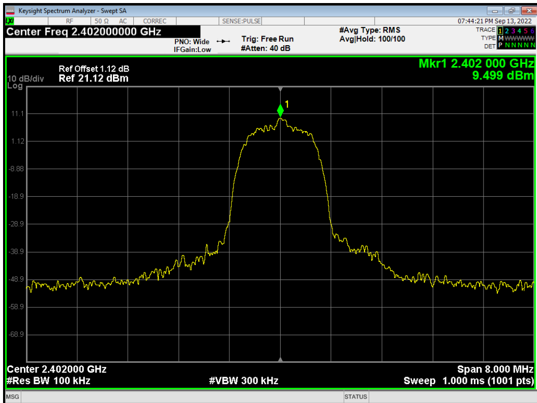
Band Edge 2-DH5 2402MHz No-Hopping Ref
