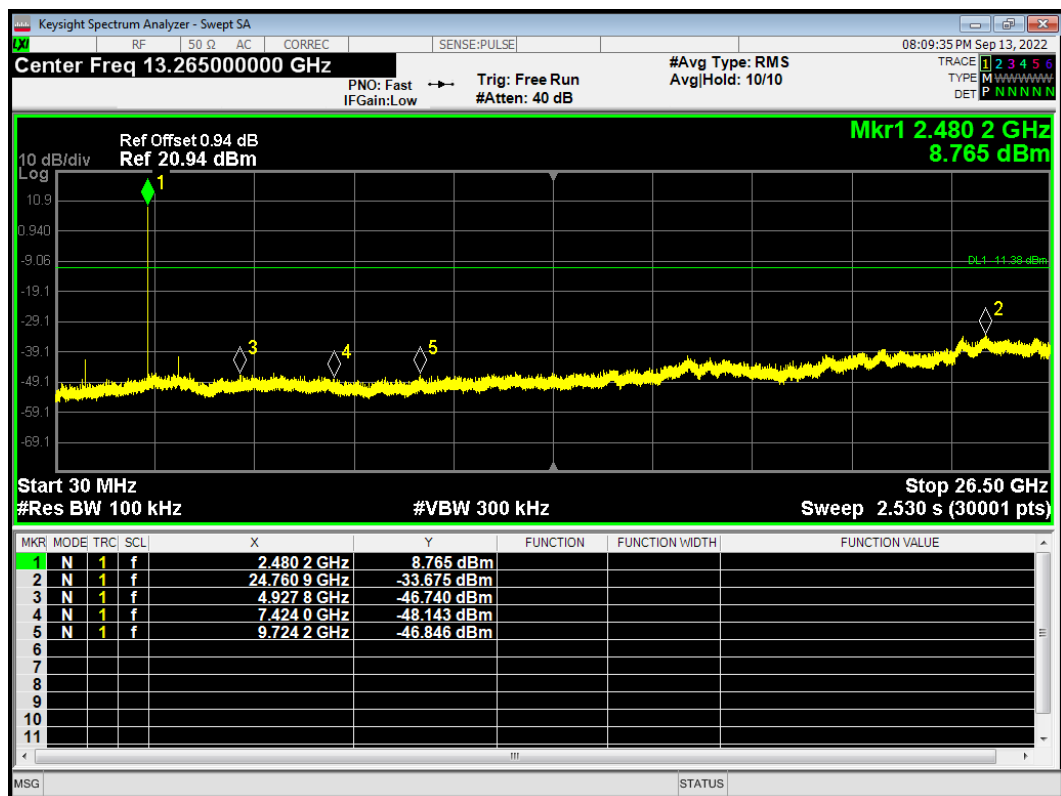
Tx. Spurious 3-DH5 2480MHz Emission
