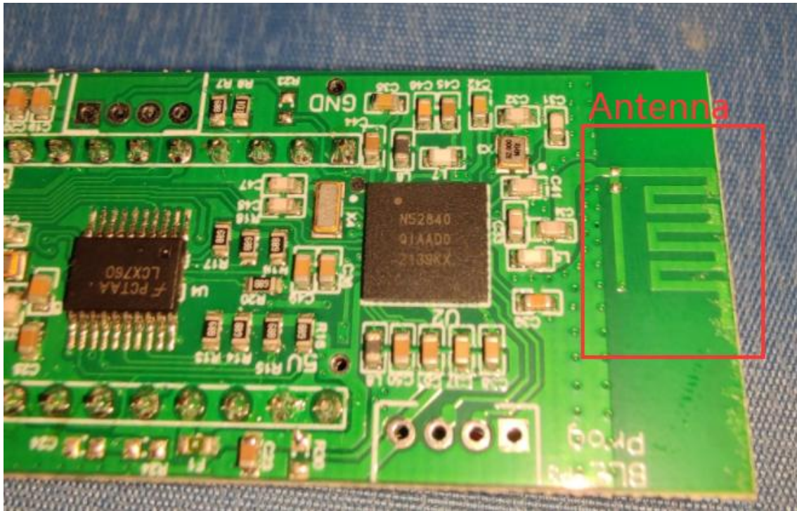
Antenna 1
