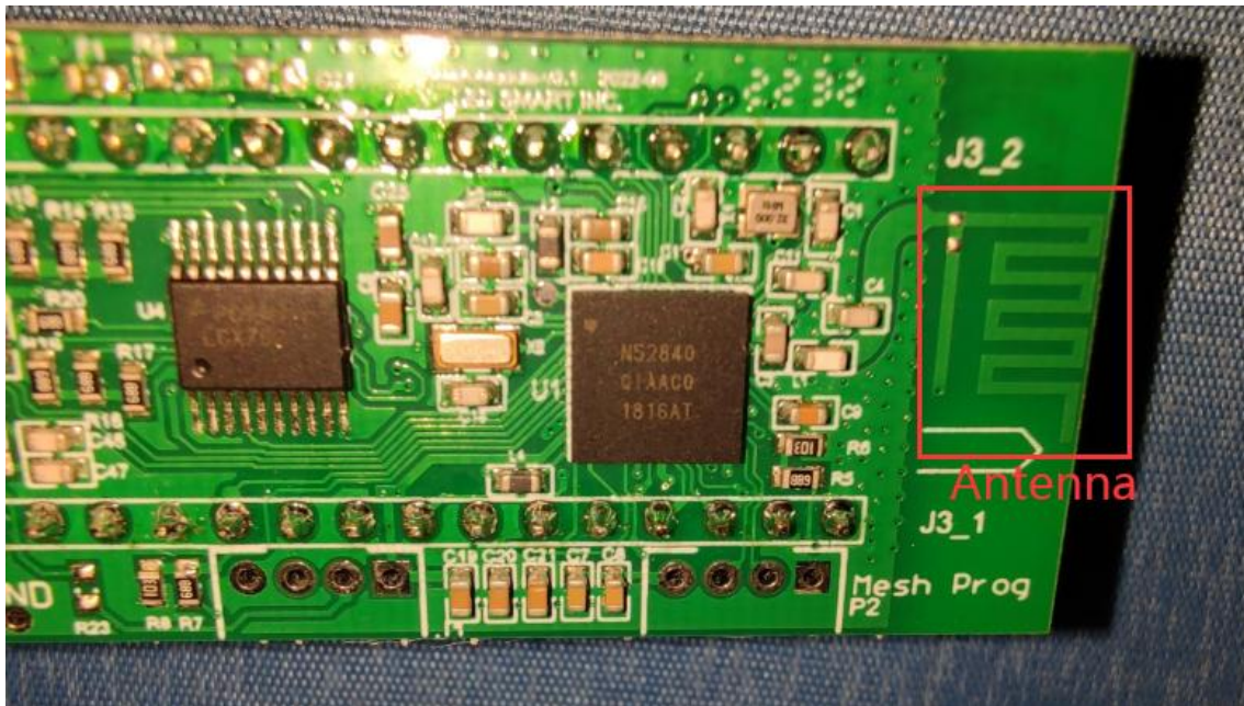
Antenna 2
