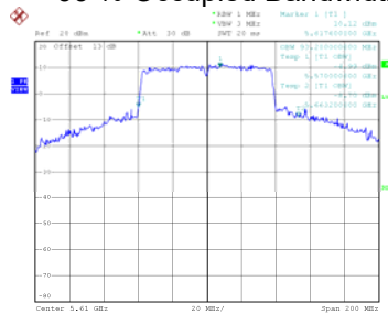
99 % Occupied Bandwidth
