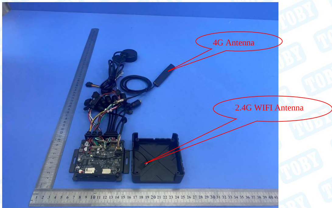
Photo 9 Internal of EUT
