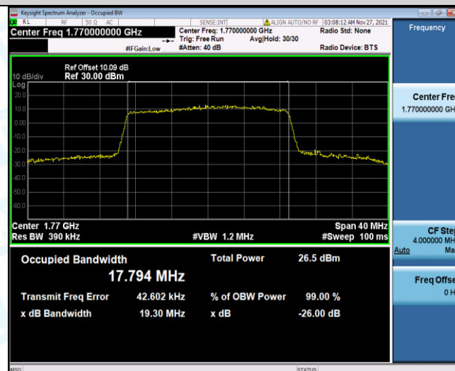
Band66-20MHz-16QAM-132572-100RB#0
