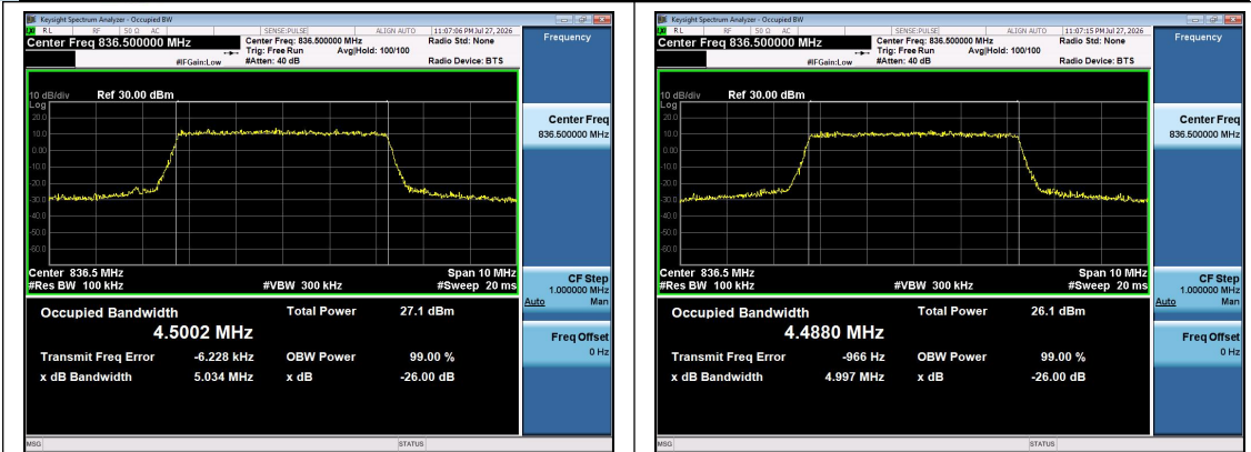
Band5-5MHz-QPSK-20525-25RB#0-PASS
