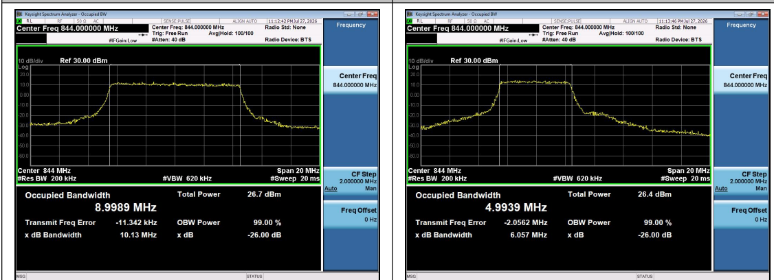
Band5-10MHz-QPSK-20600-50RB#0-PASS
