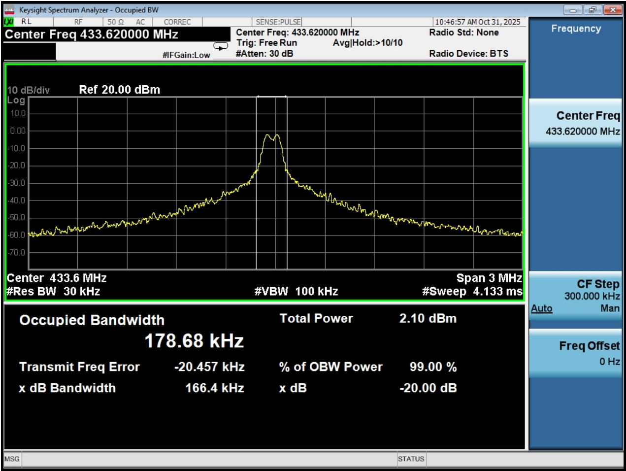
20dB Bandwidth
