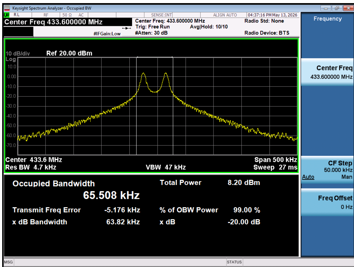
20dB Bandwidth
