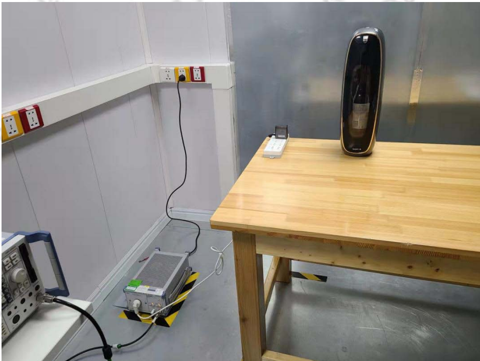
Conduction Emission
