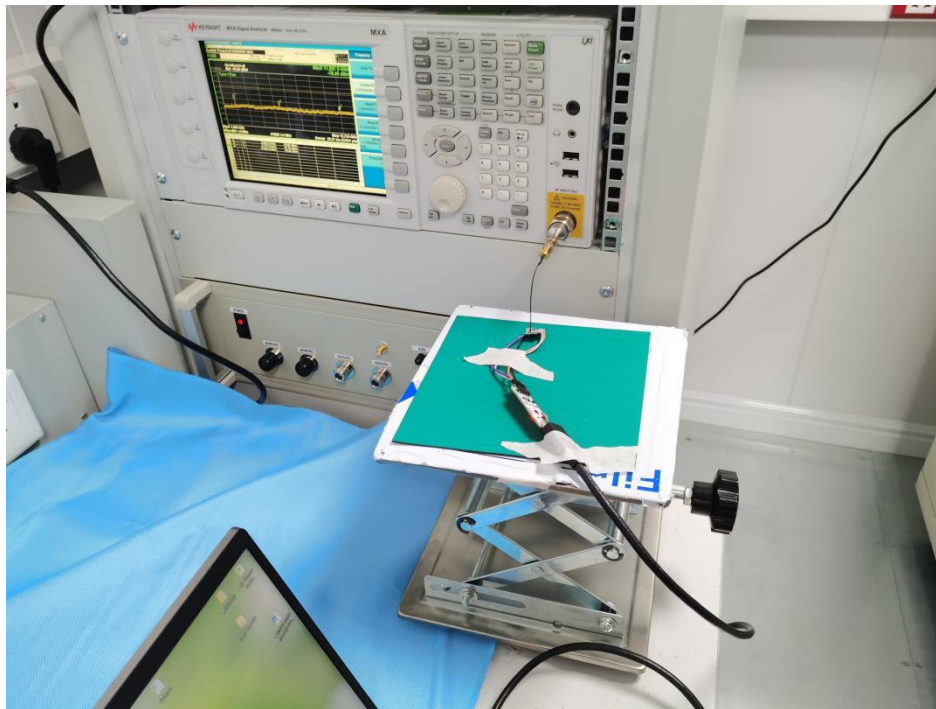
Conduction Emission
