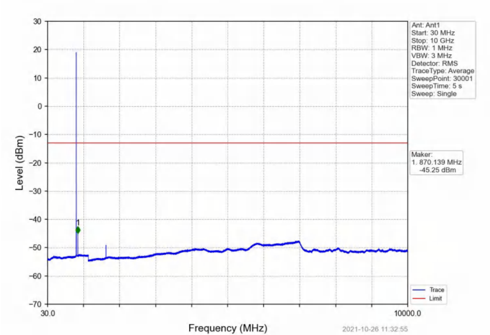
Band5_3MHz_16QAM_LCH_825.5MHz_RB_1_0_NTNV
