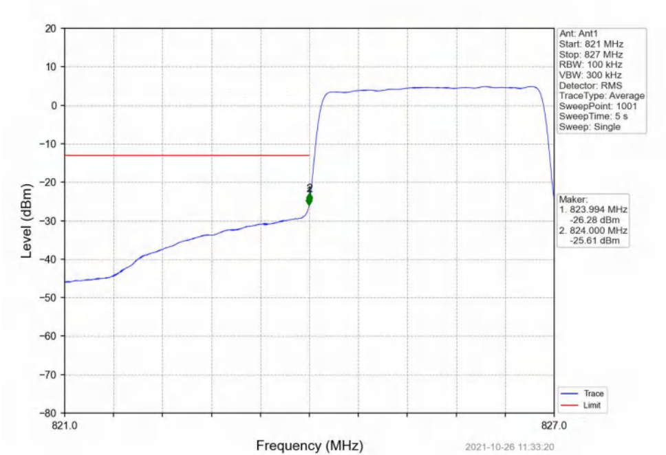
Band5_3MHz_16QAM_LCH_825.5MHz_RB_15_0_NTNV
