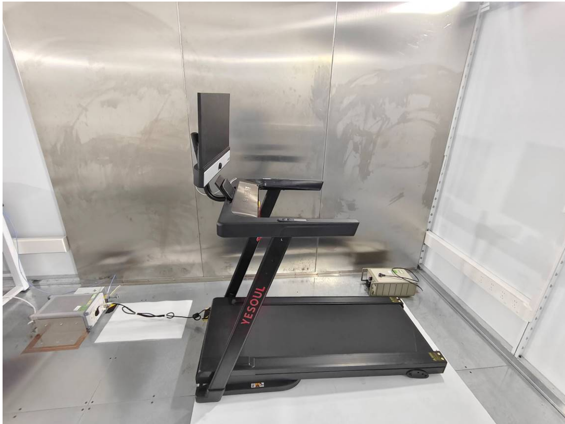
CE -Near View
