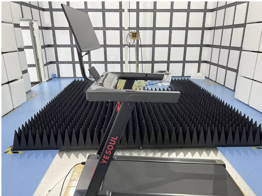
RE – Front View (1 GHz~3 GHz)
