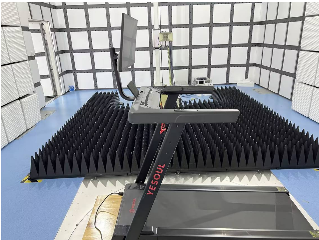
RE – Front View (3 GHz~18 GHz)
