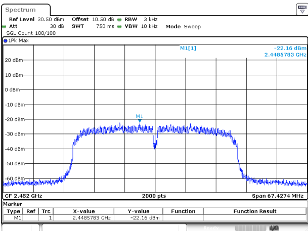
802.11n40_2452MHz
