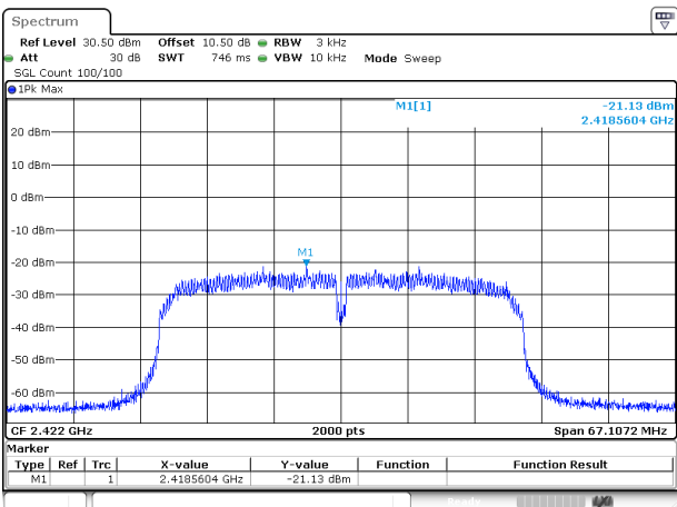
802.11n40_2422MHz
