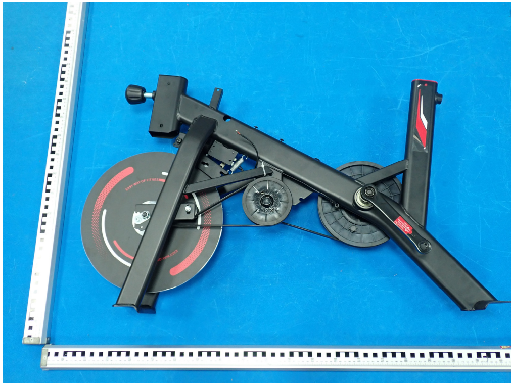
Internal Photo 3
