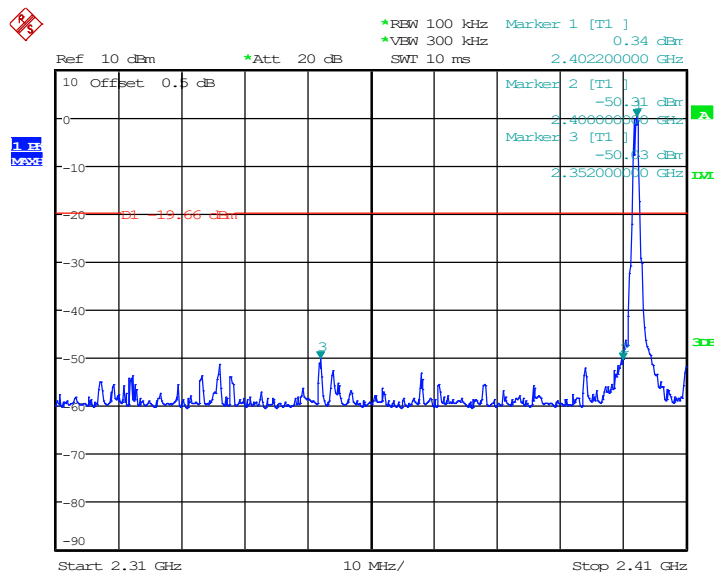
GFSK: Band Edge, Left Side
