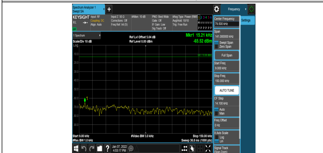
Band5-5MHz-QPSK-20625-1RB#0-Range1:0.009~0.15MHz
