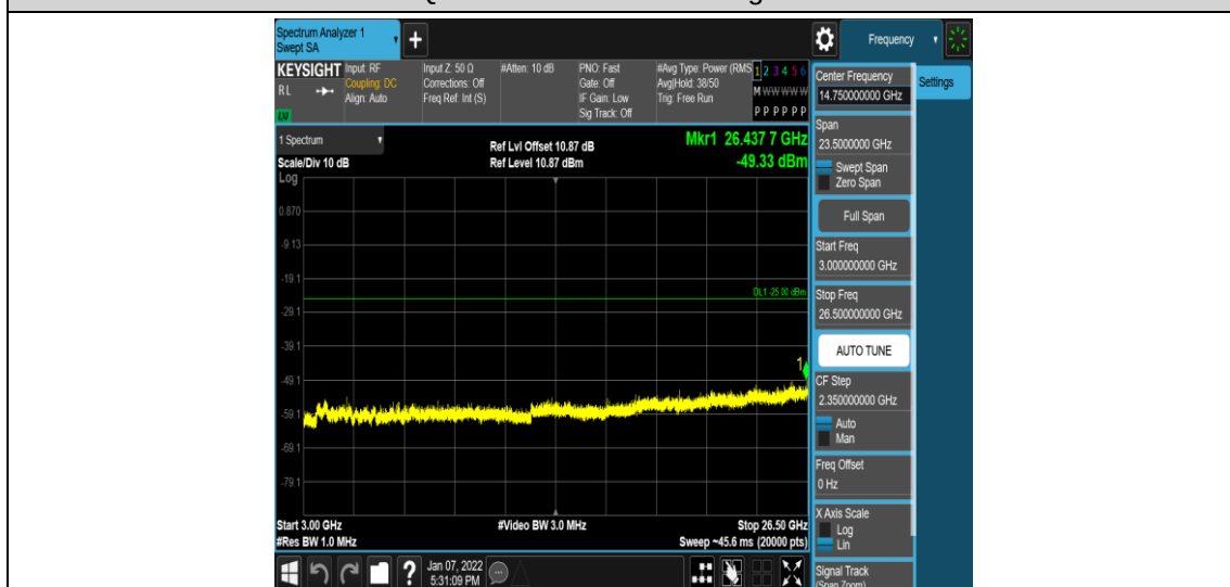
Band7-5MHz-QPSK-20775-1RB#0-Range5:3000~26500MHz
