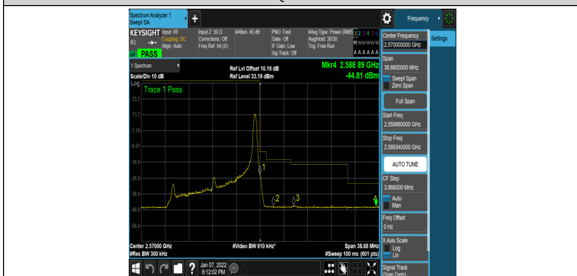
Band7-15MHz-QPSK-21375-1RB#74
