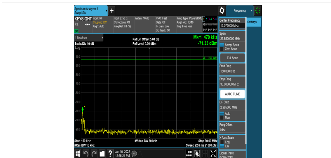
Band7-15MHz-QPSK-21375-1RB#0-Range2:0.15~30MHz
