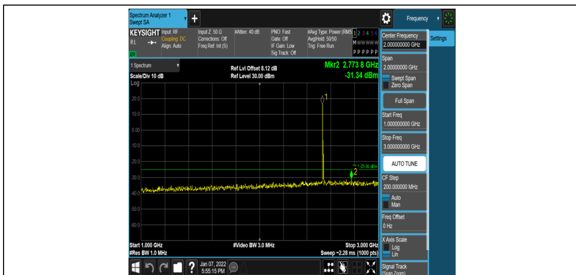
Band7-10MHz-16QAM-21100-1RB#0-Range4:1000~3000MHz
