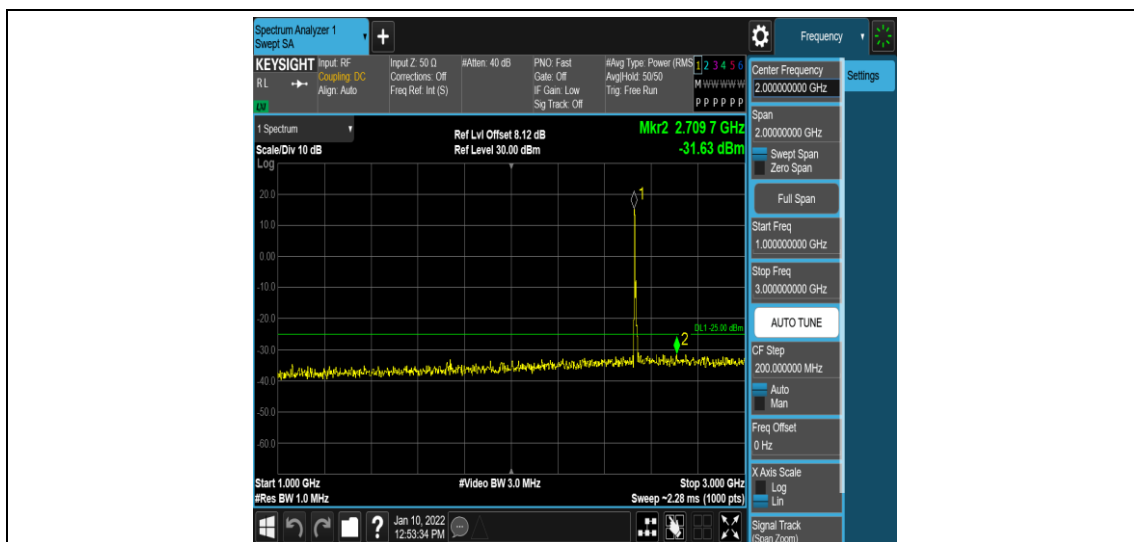
Band7-15MHz-QPSK-21100-1RB#0-Range4:1000~3000MHz
