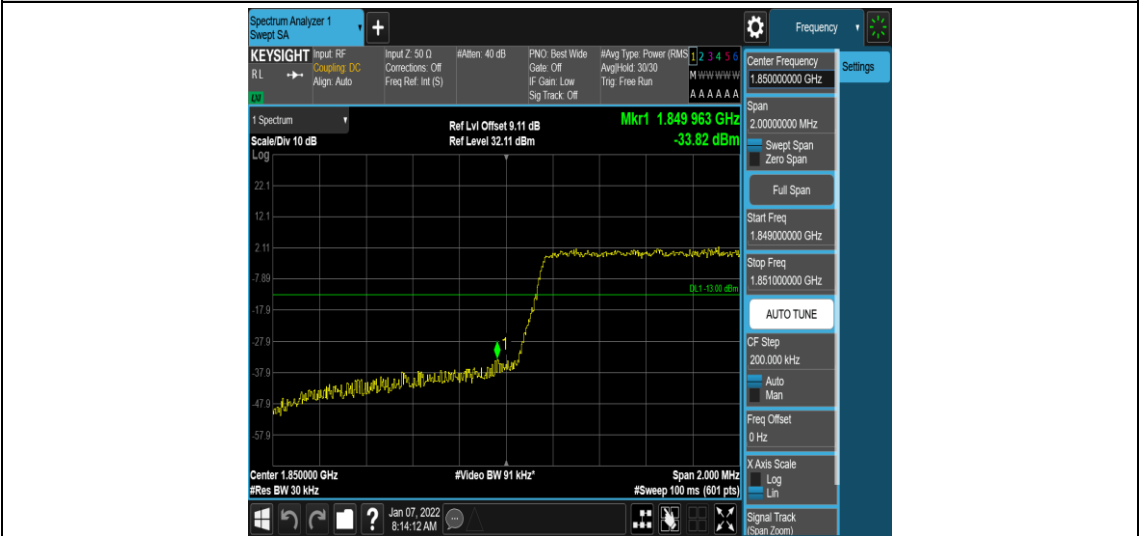
Band2-1.4MHz-QPSK-18607-6RB#0
