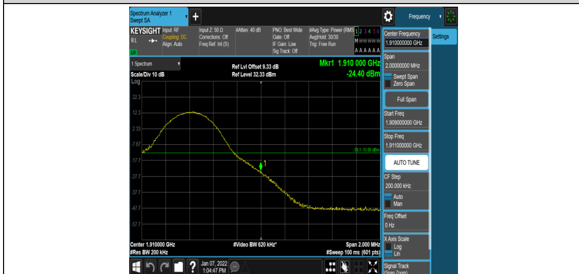
Band2-10MHz-16QAM-19150-1RB#49
