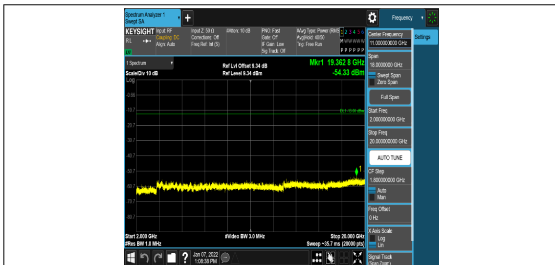
Band2-10MHz-QPSK-18900-1RB#0-Range5:2000~20000MHz
