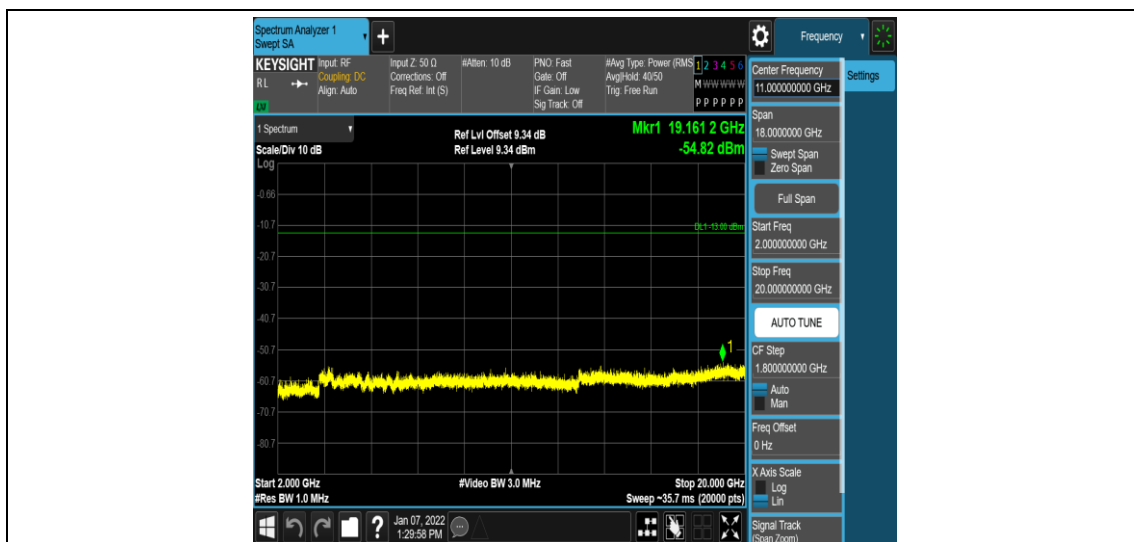
Band2-15MHz-16QAM-18900-1RB#0-Range5:2000~20000MHz
