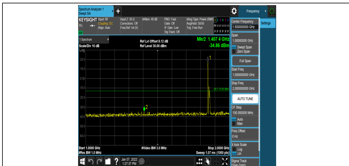
Band2-15MHz-16QAM-18675-1RB#0-Range4:1000~2000MHz
