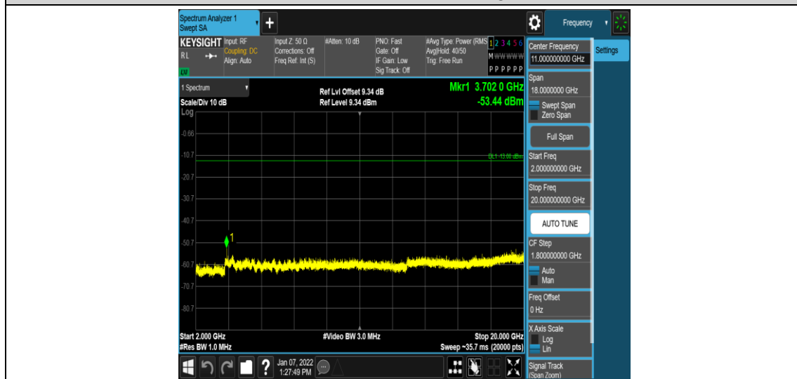
Band2-15MHz-16QAM-18675-1RB#0-Range5:2000~20000MHz
