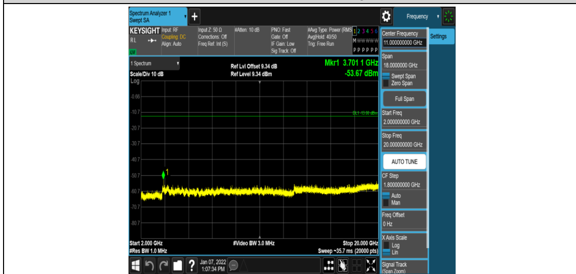
Band2-10MHz-16QAM-18650-1RB#0-Range5:2000~20000MHz
