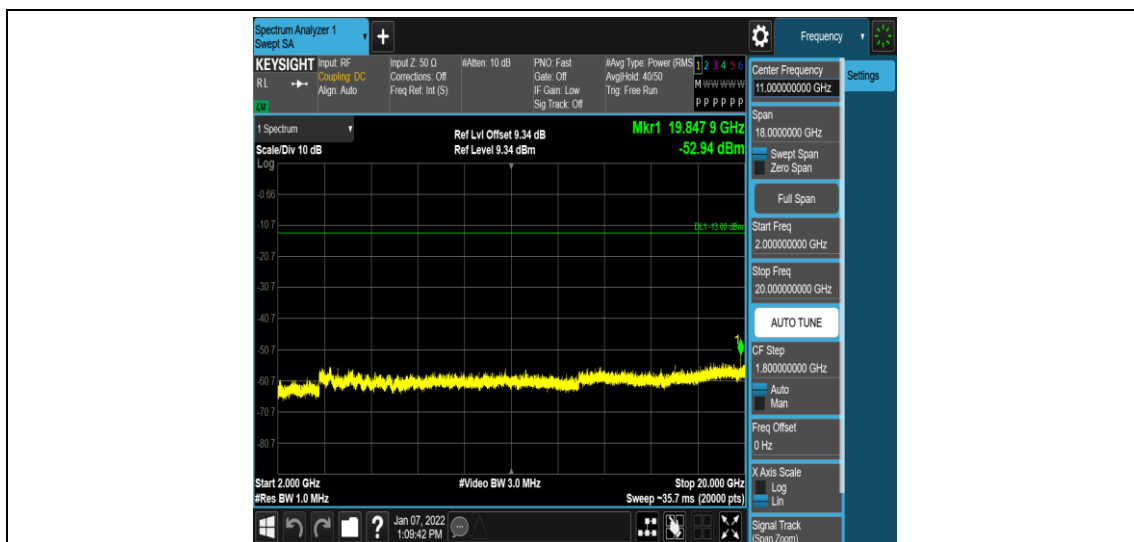
Band2-10MHz-16QAM-18900-1RB#0-Range5:2000~20000MHz
