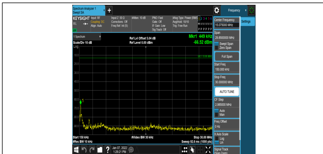
Band2-15MHz-16QAM-18900-1RB#0-Range2:0.15~30MHz
