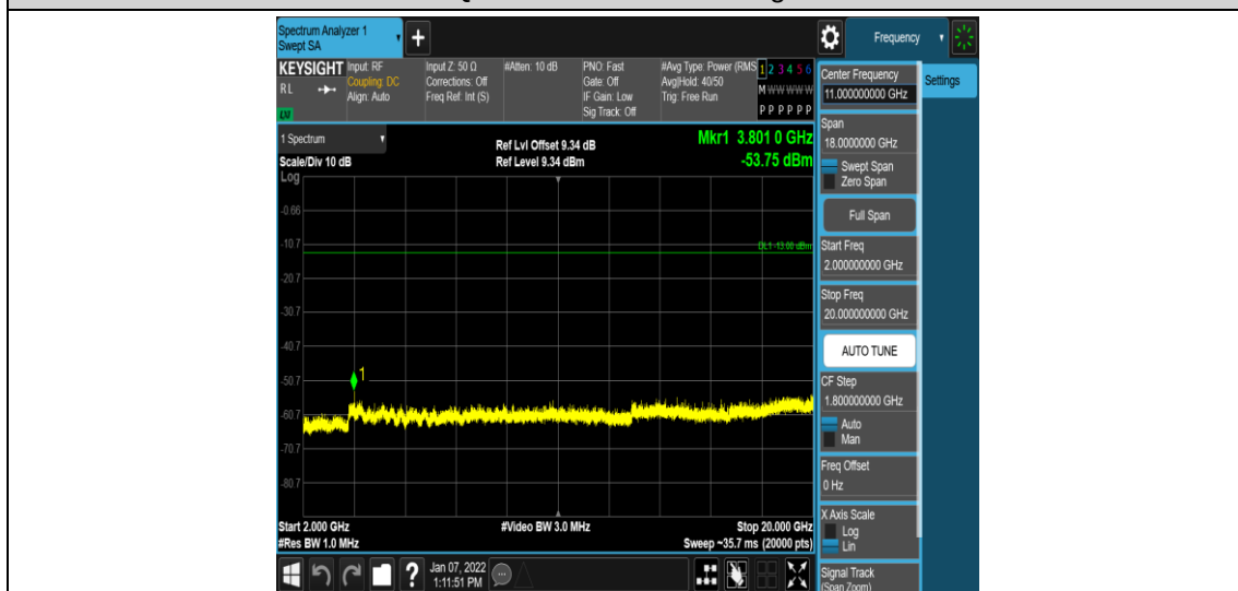
Band2-10MHz-16QAM-19150-1RB#0-Range5:2000~20000MHz
