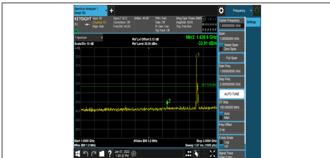
Band2-15MHz-QPSK-18675-1RB#0-Range4:1000~2000MHz
