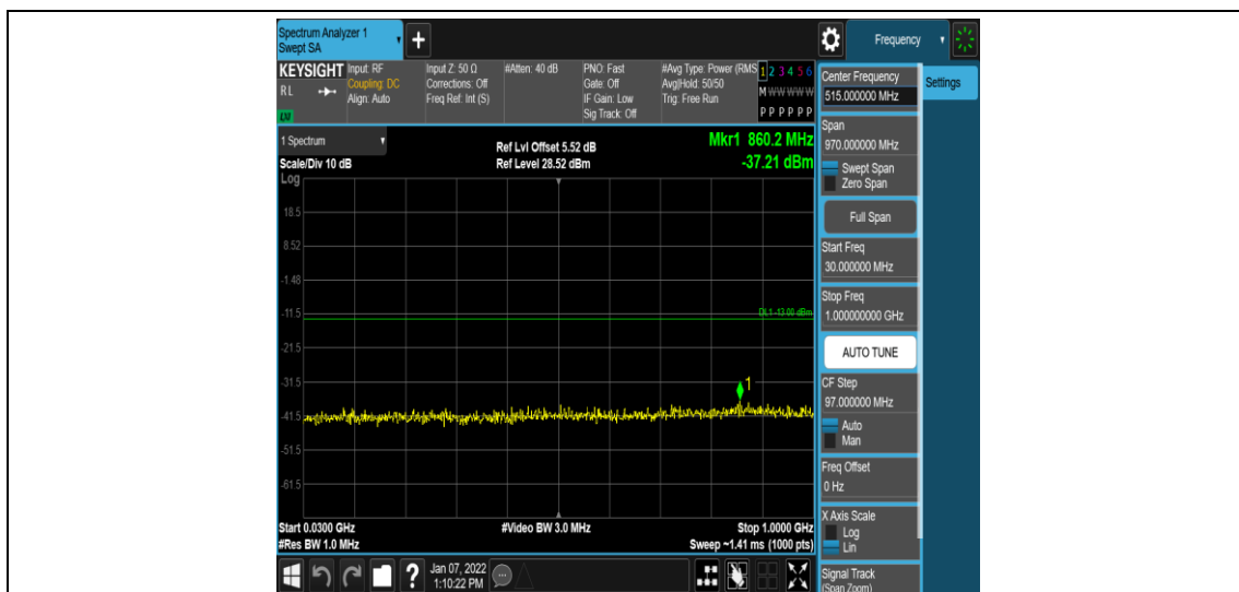
Band2-10MHz-QPSK-19150-1RB#0-Range3:30~1000MHz
