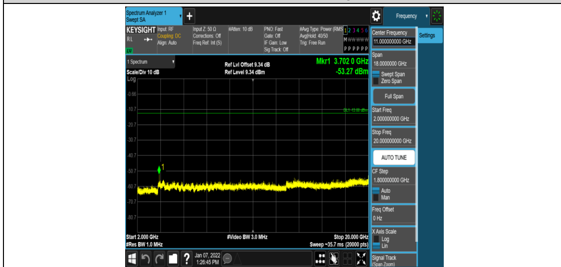
Band2-15MHz-QPSK-18675-1RB#0-Range5:2000~20000MHz
