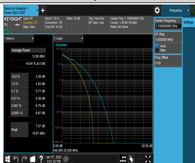
Band4-20MHz-QPSK-20300-100RB#0
