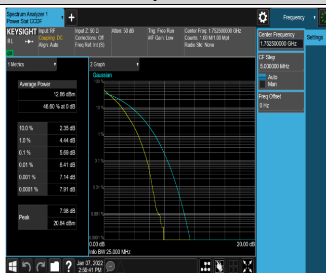
Band4-5MHz-QPSK-20375-25RB#0
