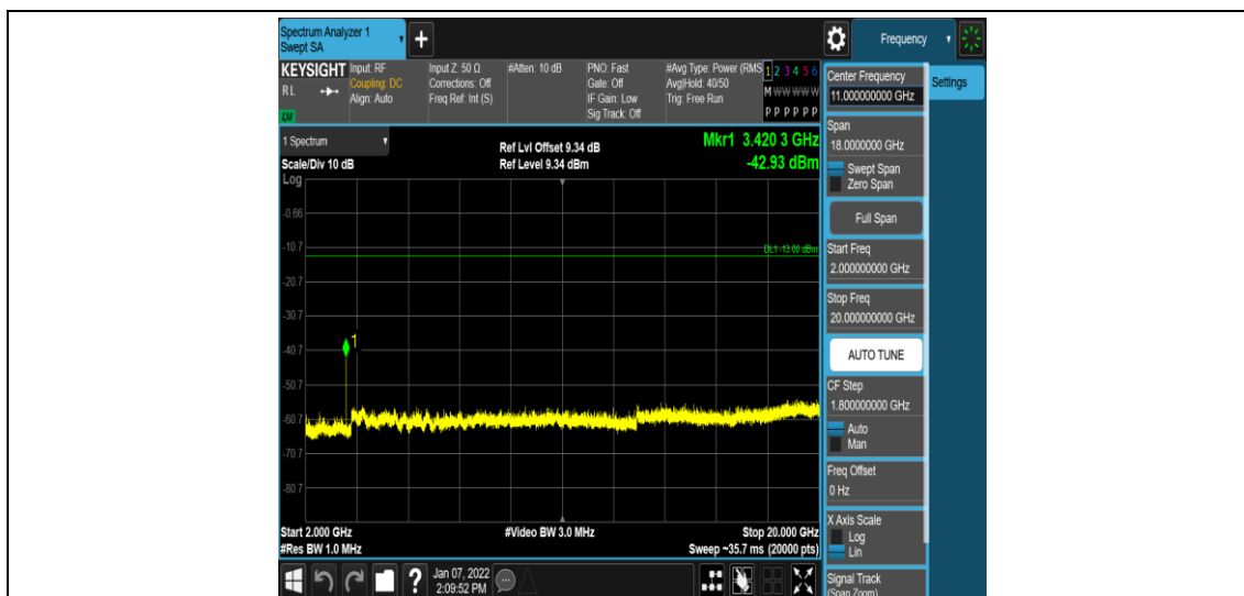
Band4-1.4MHz-16QAM-19957-1RB#0-Range5:2000~20000MHz
