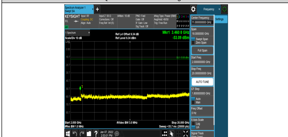
Band4-5MHz-16QAM-20175-1RB#0-Range5:2000~20000MHz
