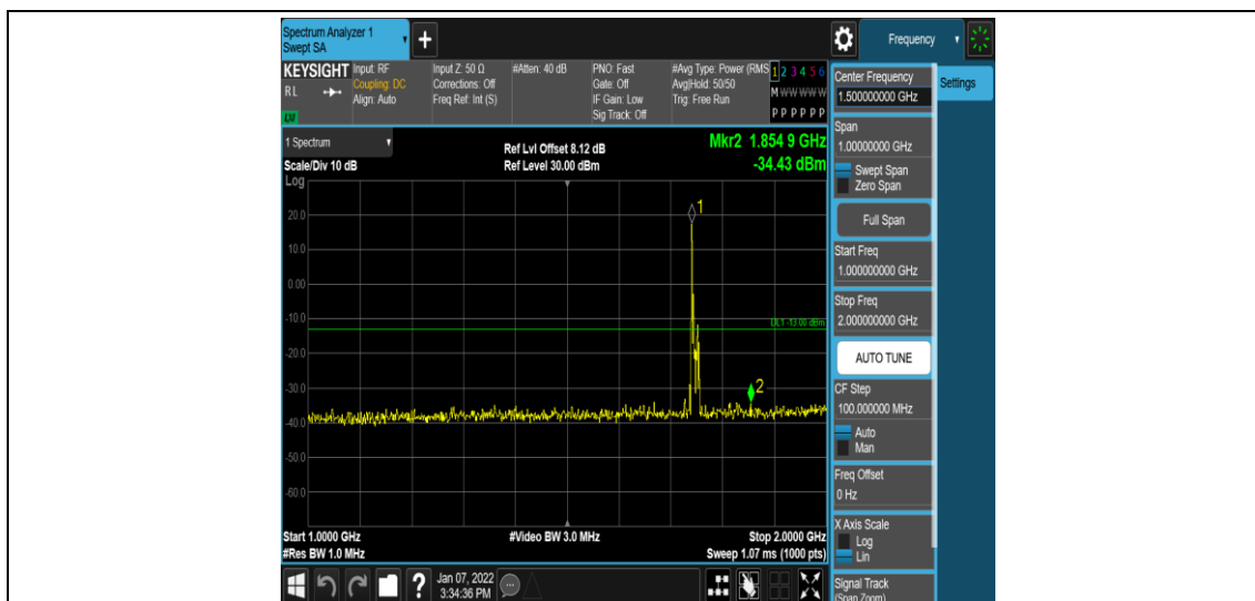
Band4-15MHz-QPSK-20325-1RB#0-Range4:1000~2000MHz
