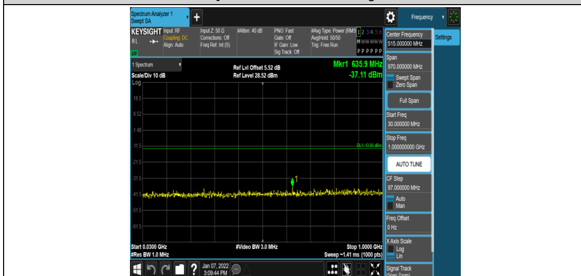
Band4-10MHz-QPSK-20000-1RB#0-Range3:30~1000MHz
