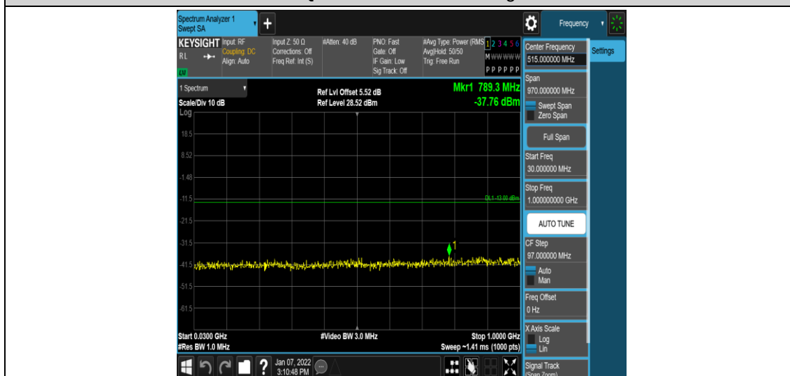
Band4-10MHz-16QAM-20000-1RB#0-Range3:30~1000MHz
