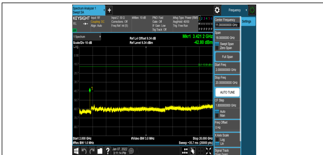
Band4-10MHz-16QAM-20000-1RB#0-Range5:2000~20000MHz
