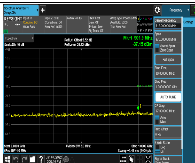
Band4-15MHz-QPSK-20175-1RB#0-Range3:30~1000MHz
