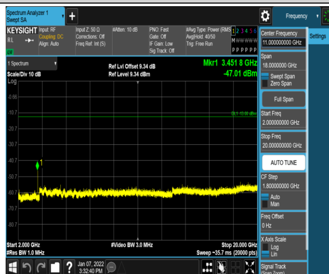
Band4-15MHz-QPSK-20175-1RB#0-Range5:2000~20000MHz
