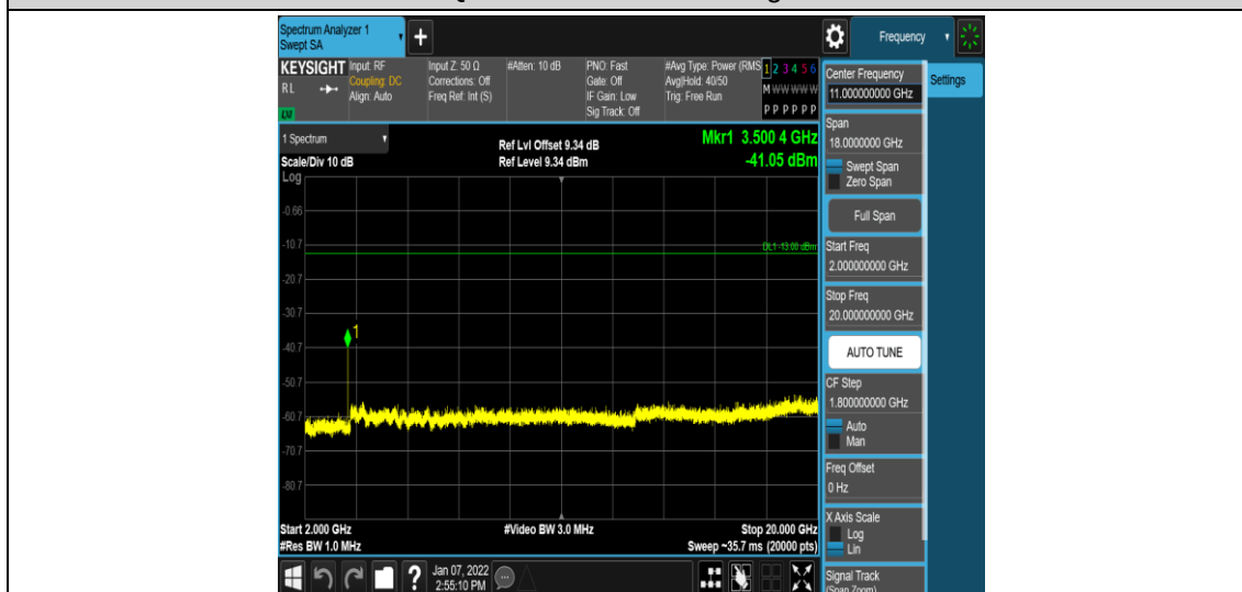
Band4-5MHz-16QAM-20375-1RB#0-Range5:2000~20000MHz
