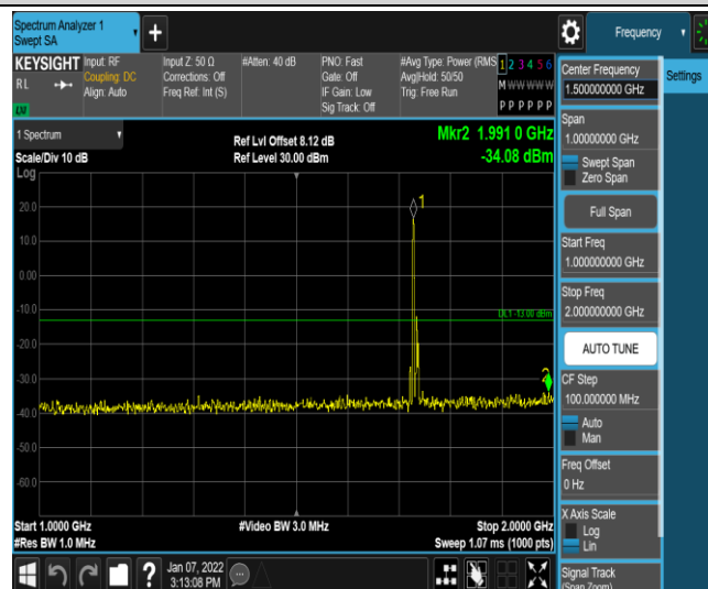
Band4-10MHz-16QAM-20175-1RB#0-Range4:1000~2000MHz
