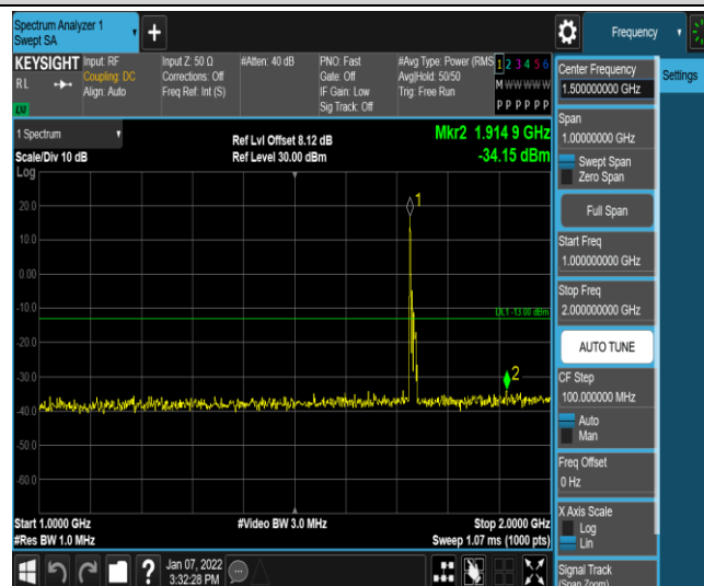
Band4-15MHz-QPSK-20175-1RB#0-Range4:1000~2000MHz
