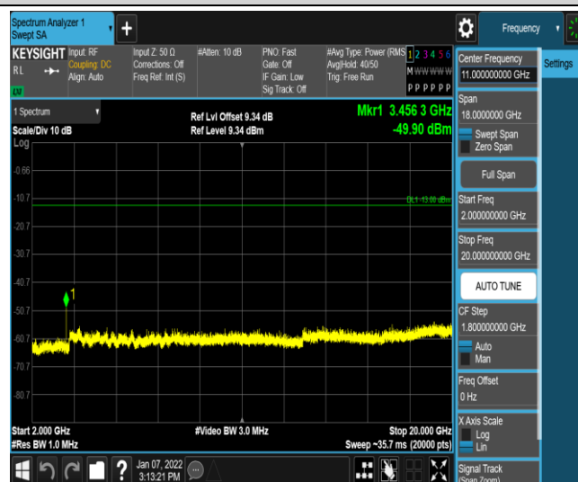
Band4-10MHz-16QAM-20175-1RB#0-Range5:2000~20000MHz
