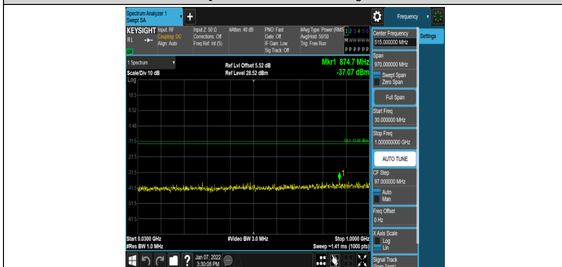
Band4-15MHz-QPSK-20025-1RB#0-Range3:30~1000MHz
