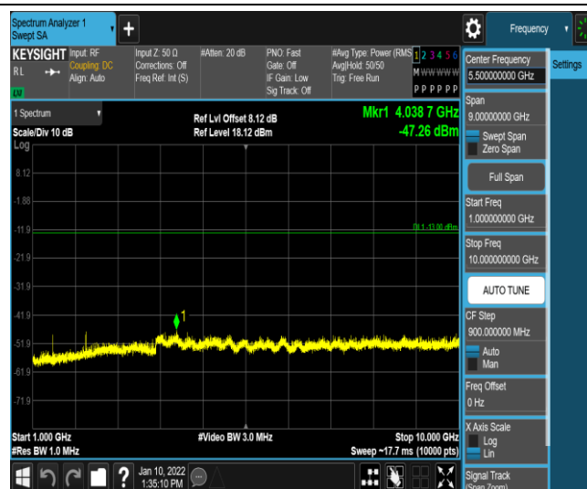
Band12-1.4MHz-QPSK-23095-1RB#0-Range4:1000~10000MHz
