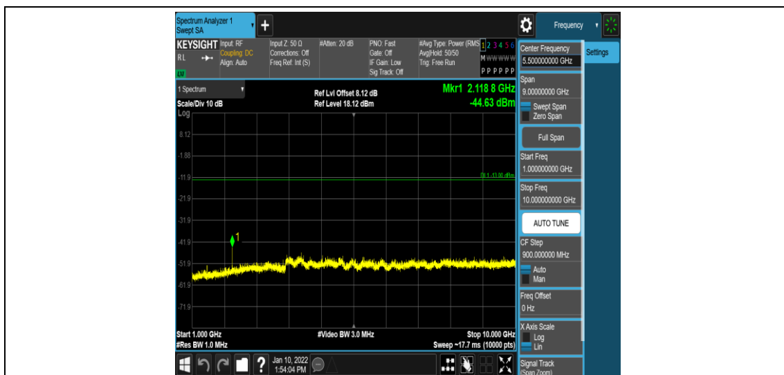
Band12-3MHz-QPSK-23095-1RB#0-Range4:1000~10000MHz
