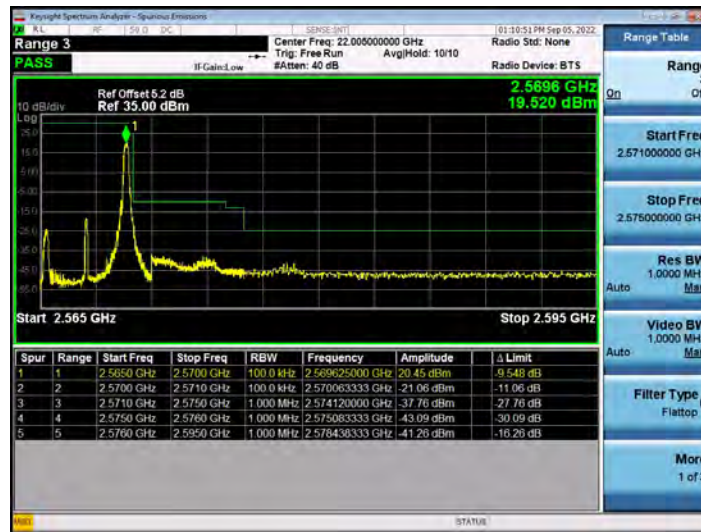
Band7-5MHz-QPSK-21425-25RB#0
