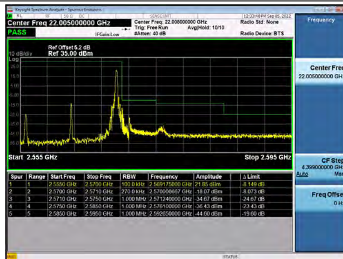
Band7-15MHz-QPSK-21375-1RB#74
