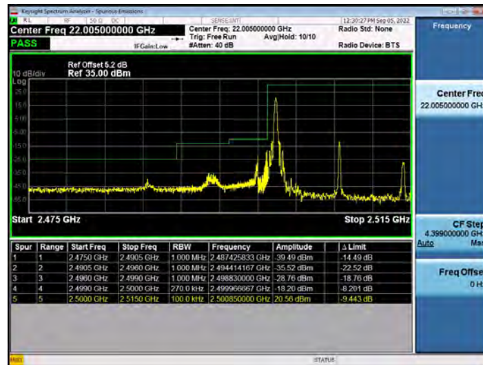
Band7-15MHz-QPSK-20825-75RB#0
