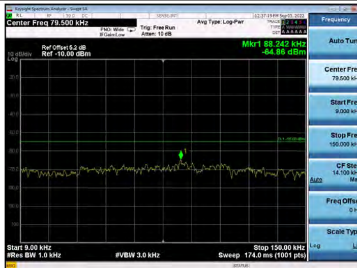
Band7-20MHz-QPSK-21100-1RB#0-Range1: 9KHz~150KHz
