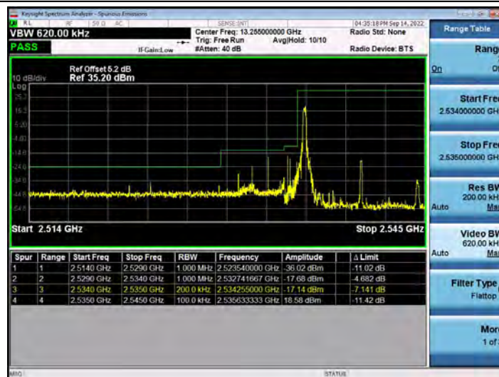
Band41-10MHz-QPSK-40090-1RB#0
