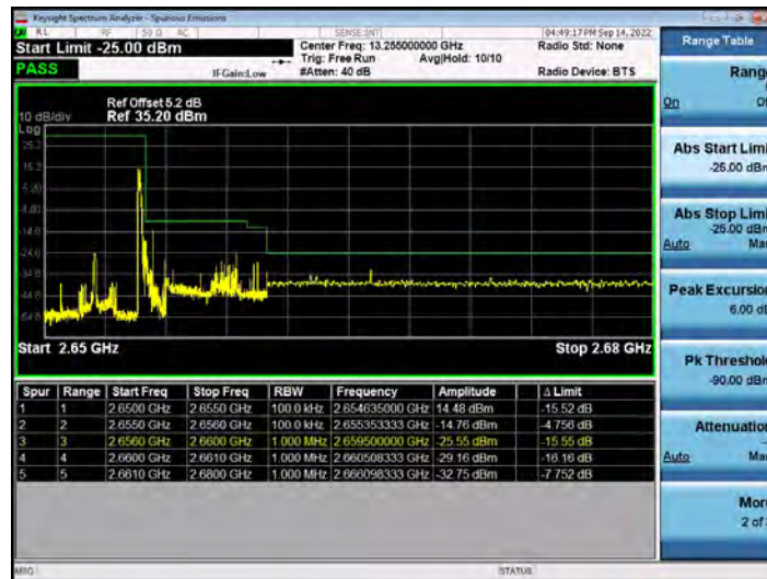
Band41-5MHz-QPSK-41215-25RB#0
