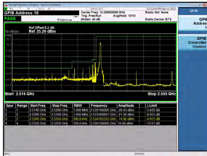
Band41-20MHz-QPSK-40140-100RB#0
