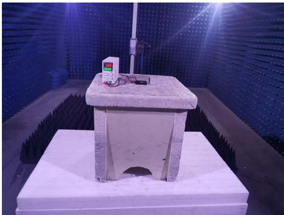
Photo of Radiated Emission Measurement 1-18GHz
