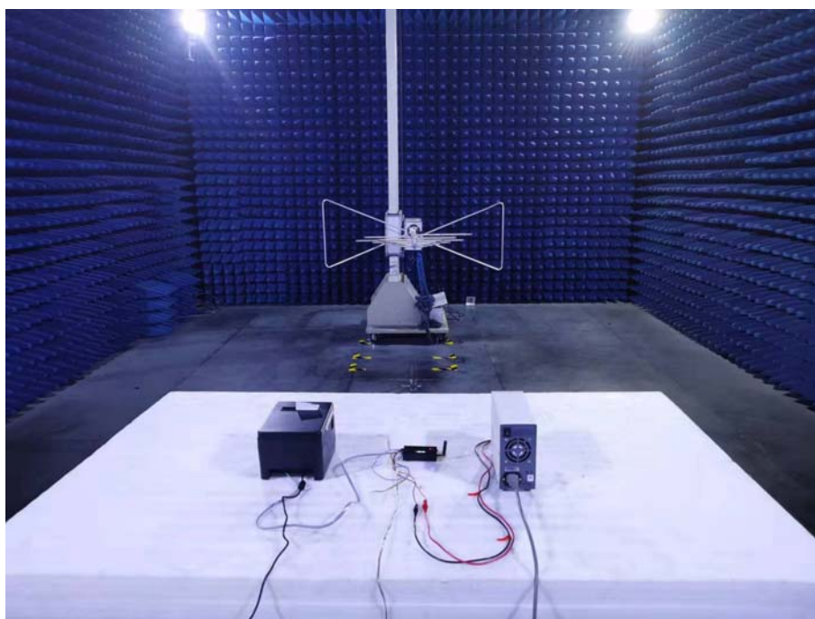
Photo of Radiated Emission Measurement Below 1GHz - Side View
