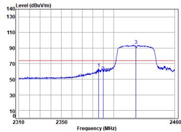
11n_HT(40M)_TX_CH_03_Horizontal-Peak
