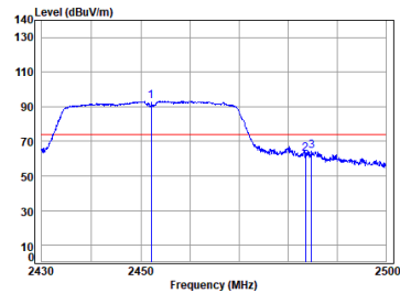
11n_HT(40M)_TX_CH_09_Horizontal-Peak
