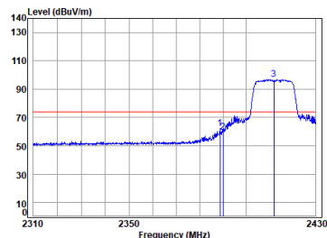
11n_HT(20M)_TX_CH_01_Horizontal-Peak
