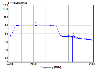
11n_HT(40M)_TX_CH_09_Vertical-Peak
