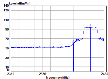
11n_HT(20M)_TX_CH_01_Vertical-Peak
