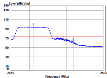
11n_HT(20M)_TX_CH_11_Vertical-Peak
