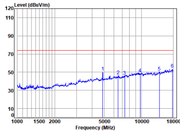
11n_HT(20M)_TX_CH_06_Vertical-Peak
