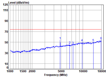
11b_TX_CH_06_Horizontal-Peak
