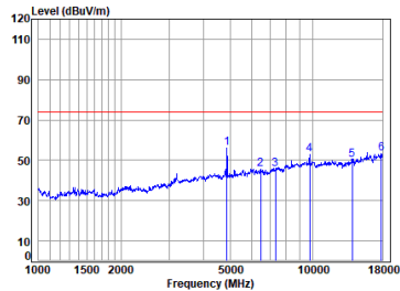
11b_TX_CH_06_Vertical-Peak
