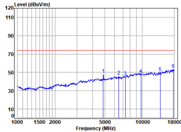
11n_HT(20M)_TX_CH_06_Horizontal-Peak
