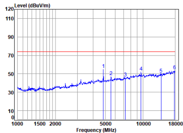
11b_TX_CH_01_Vertical-Peak
