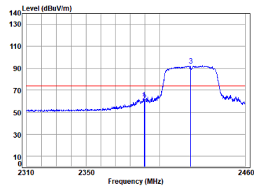
11n_HT(40M)_TX_CH_03_Vertical-Peak
