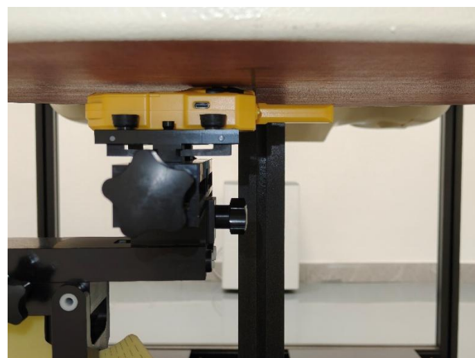
Body-worn Front (0mm)
