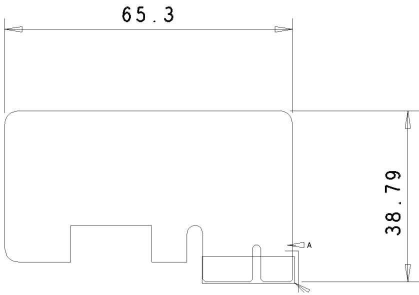
Board Outlines
