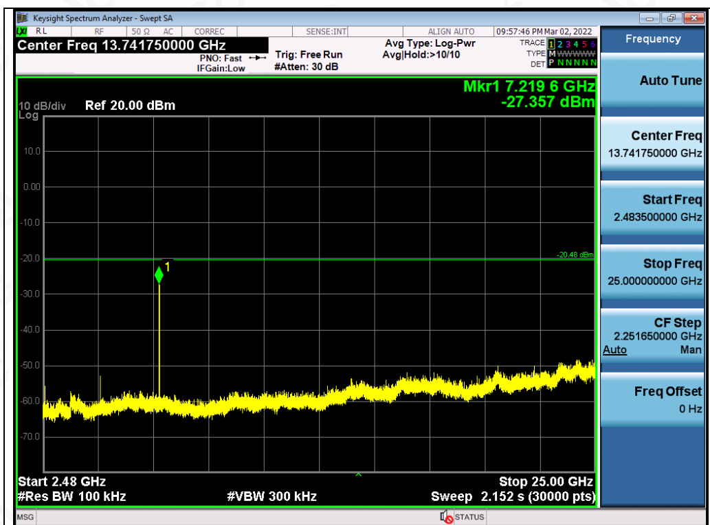
Test_Graph_LE1M_ANT1_2407_1Mbps_Higher Band Emissions
