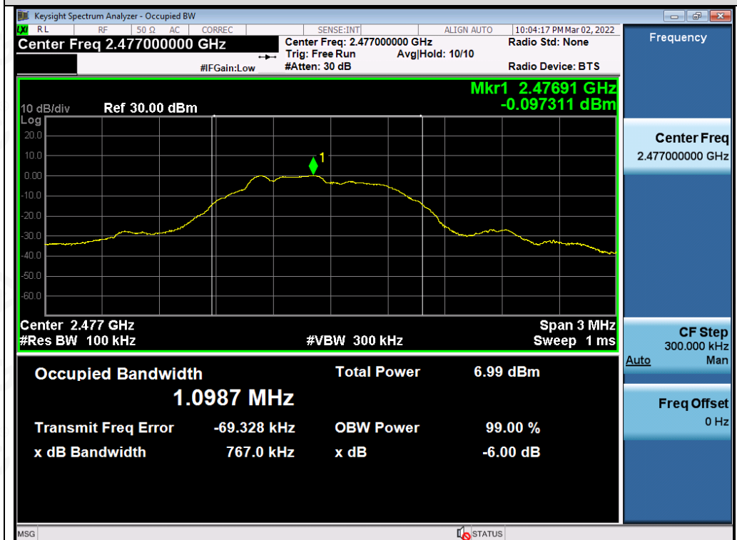
Test_Graph_LE1M_ANT1_2477_1Mbps_DTSBW
